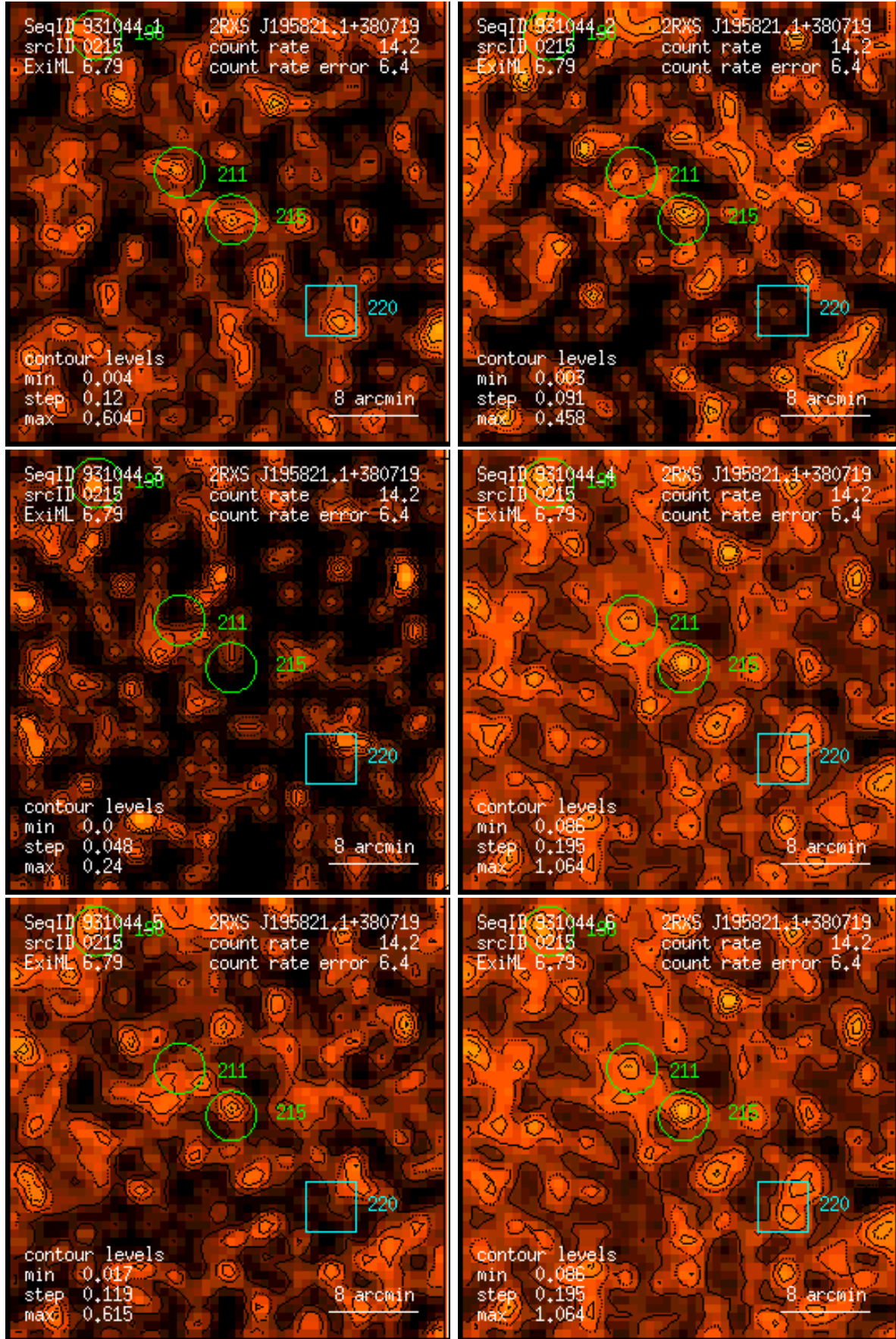
Figure 215: RASS 931044: detection 0215: band rate images, Gaussian filter: (1) PSPC channels 11 – 41, (2) 52 – 90, (3) 91 – 201, (4) 11 – 235, (5) 52 – 201, (6) 11 – 201. Broad band rates in counts/ks. Band rate contour levels in counts/ks/arcmin 2 .
