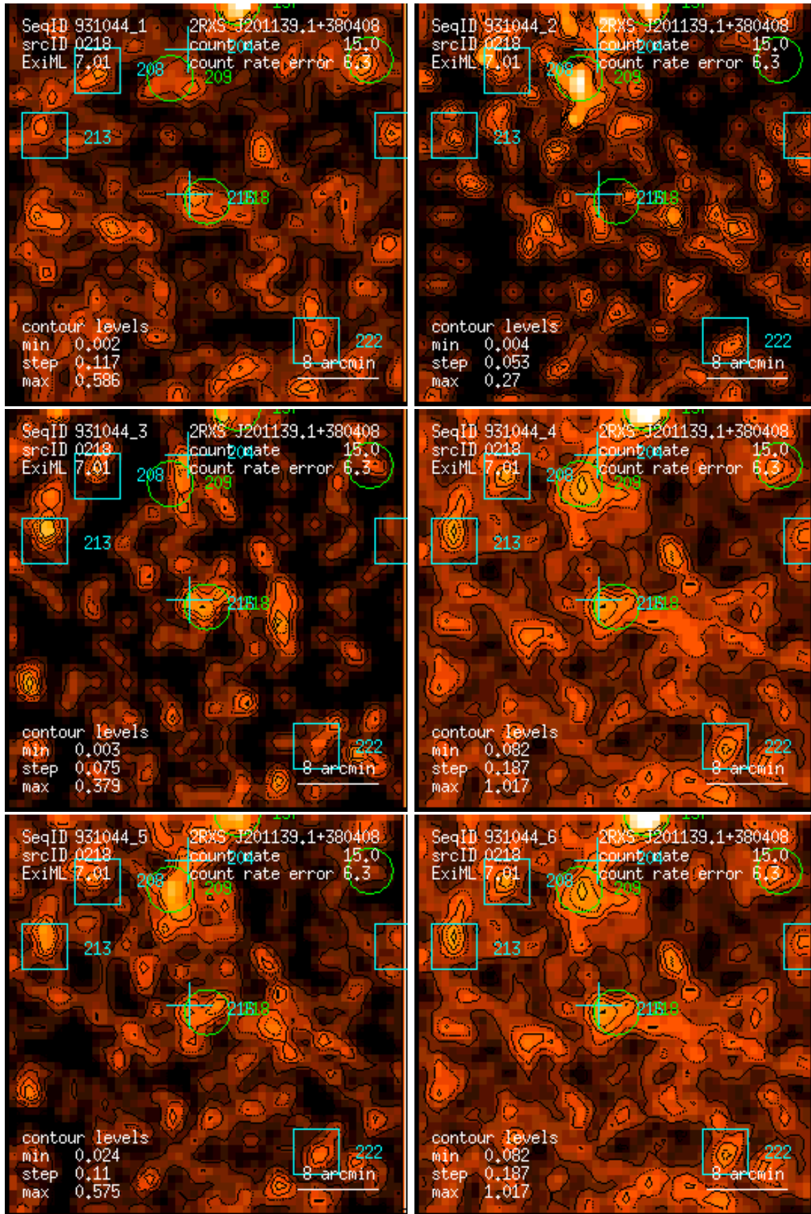
Figure 218: RASS 931044: detection 0218: band rate images, Gaussian filter: (1) PSPC channels 11 – 41, (2) 52 – 90, (3) 91 – 201, (4) 11 – 235, (5) 52 – 201, (6) 11 – 201. Broad band rates in counts/ks. Band rate contour levels in counts/ks/arcmin 2 .
