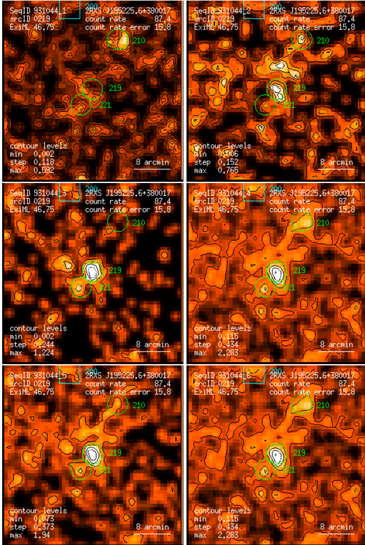
Figure 219: RASS 931044: detection 0219: band rate images, Gaussian filter: (1) PSPC channels 11 – 41, (2) 52 – 90, (3) 91 – 201, (4) 11 – 235, (5) 52 – 201, (6) 11 – 201. Broad band rates in counts/ks. Band rate contour levels in counts/ks/arcmin 2 .
