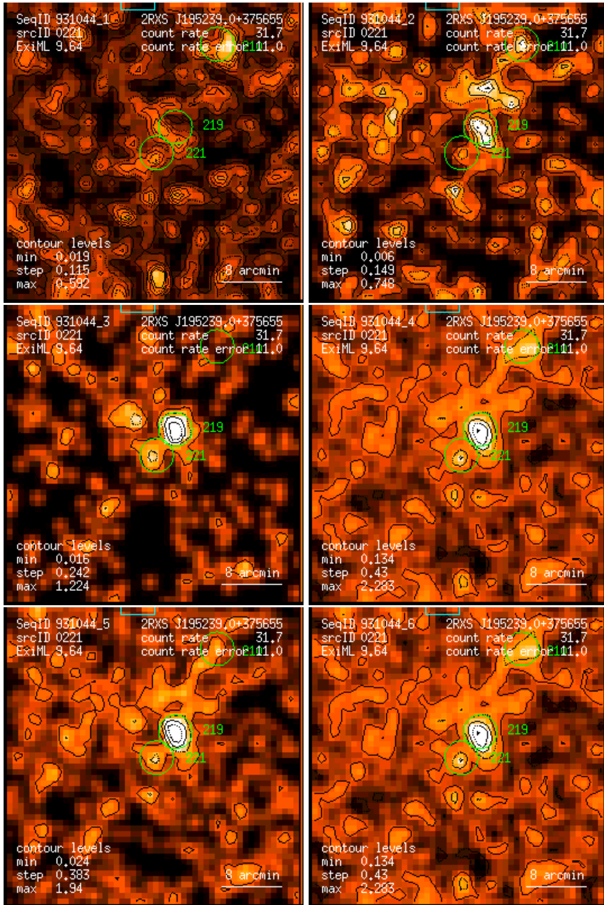
Figure 221: RASS 931044: detection 0221: band rate images, Gaussian filter: (1) PSPC channels 11 – 41, (2) 52 – 90, (3) 91 – 201, (4) 11 – 235, (5) 52 – 201, (6) 11 – 201. Broad band rates in counts/ks. Band rate contour levels in counts/ks/arcmin 2 .
