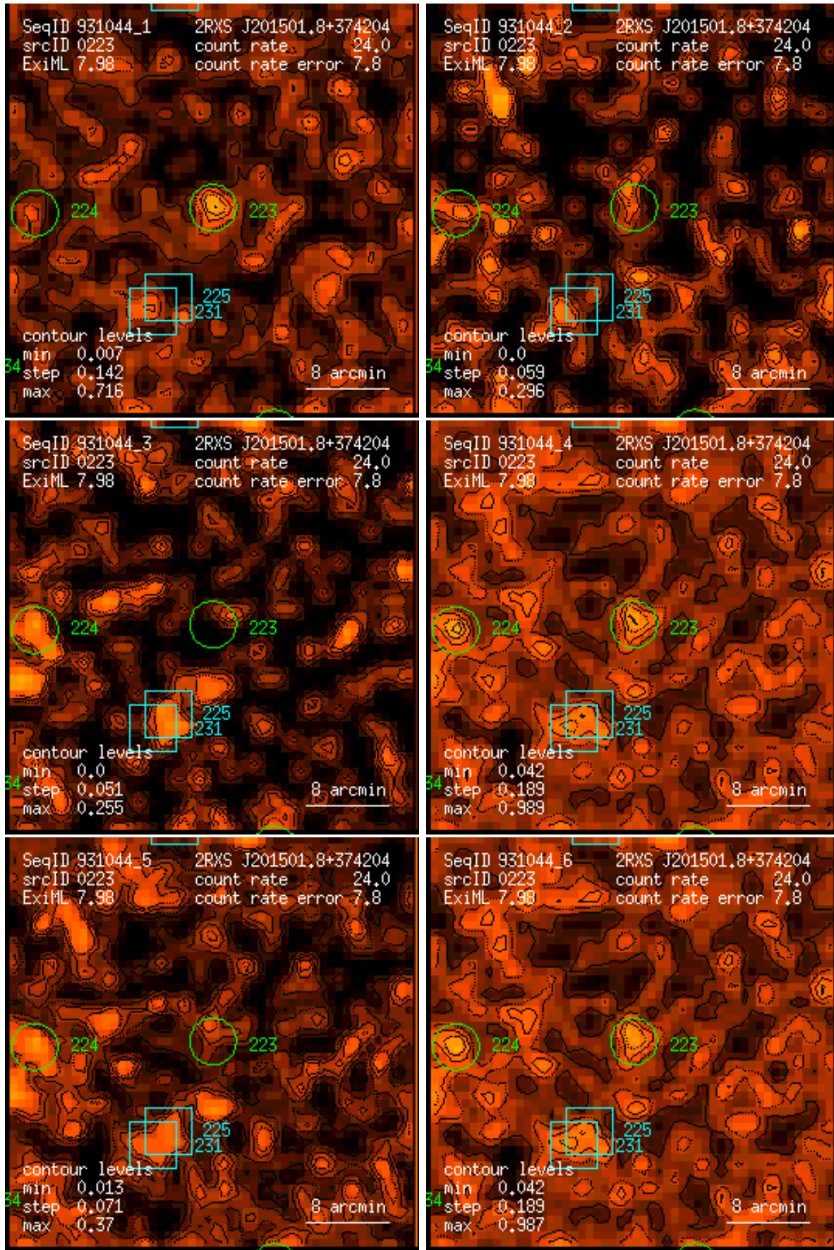
Figure 223: RASS 931044: detection 0223: band rate images, Gaussian filter: (1) PSPC channels 11 – 41, (2) 52 – 90, (3) 91 – 201, (4) 11 – 235, (5) 52 – 201, (6) 11 – 201. Broad band rates in counts/ks. Band rate contour levels in counts/ks/arcmin 2 .
