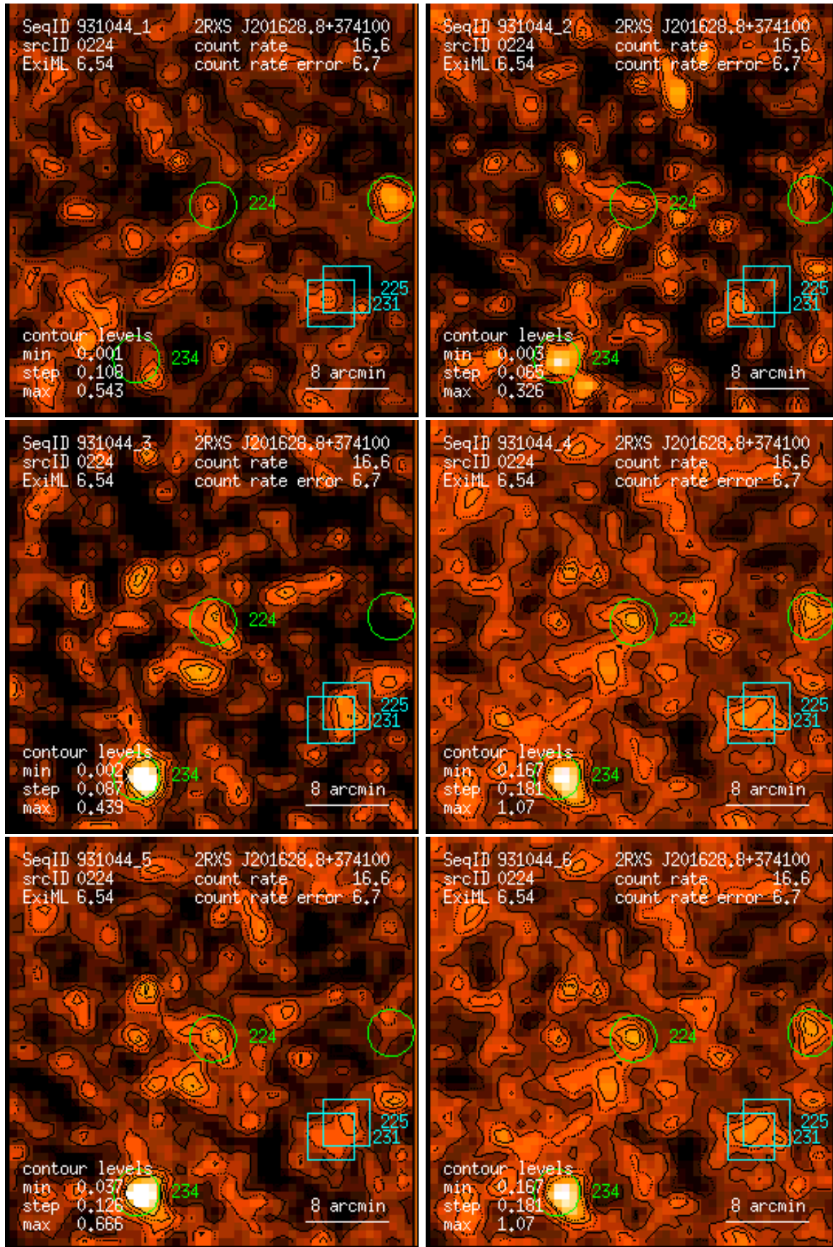
Figure 224: RASS 931044: detection 0224: band rate images, Gaussian filter: (1) PSPC channels 11 – 41, (2) 52 – 90, (3) 91 – 201, (4) 11 – 235, (5) 52 – 201, (6) 11 – 201. Broad band rates in counts/ks. Band rate contour levels in counts/ks/arcmin 2 .
