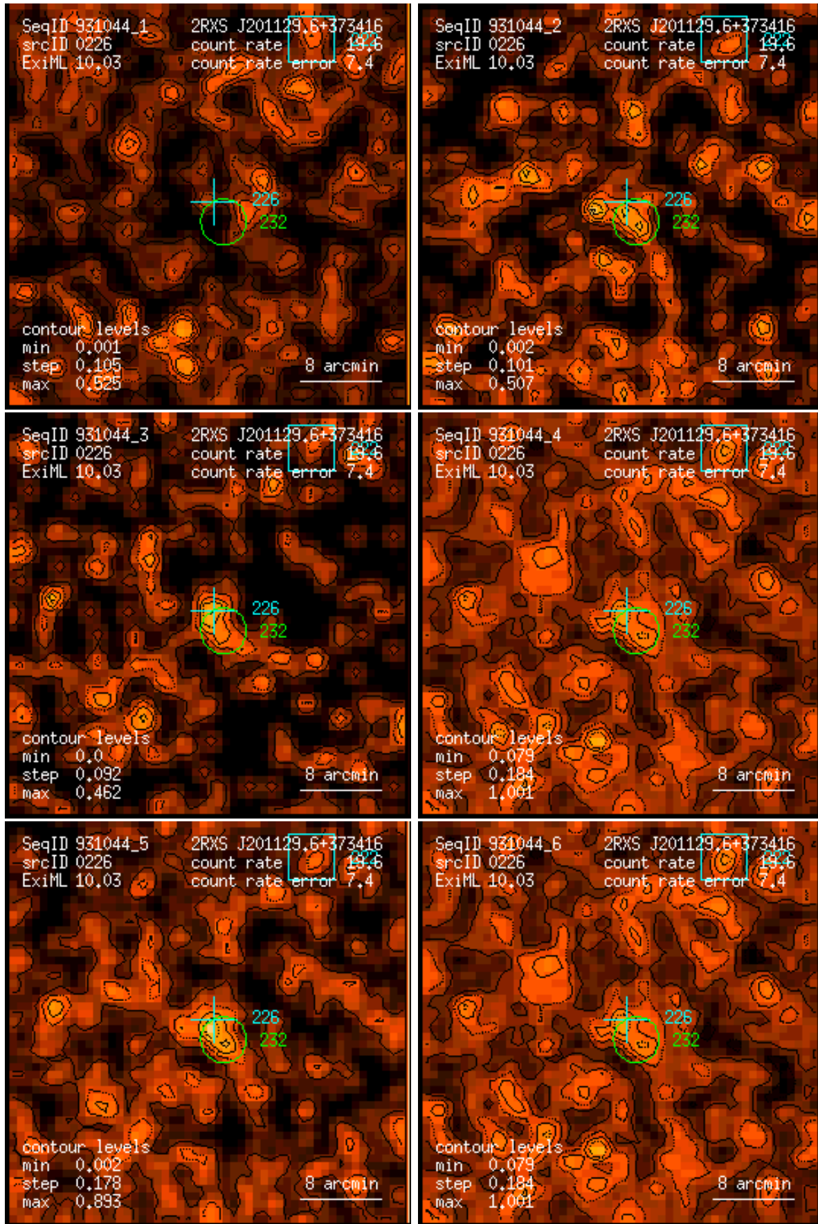
Figure 226: RASS 931044: detection 0226: band rate images, Gaussian filter: (1) PSPC channels 11 – 41, (2) 52 – 90, (3) 91 – 201, (4) 11 – 235, (5) 52 – 201, (6) 11 – 201. Broad band rates in counts/ks. Band rate contour levels in counts/ks/arcmin 2 .
