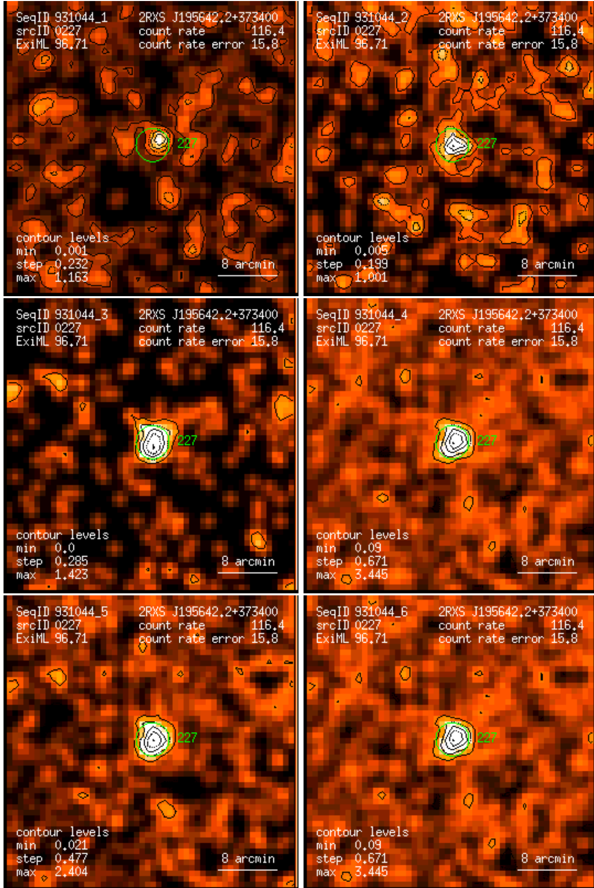
Figure 227: RASS 931044: detection 0227: band rate images, Gaussian filter: (1) PSPC channels 11 – 41, (2) 52 – 90, (3) 91 – 201, (4) 11 – 235, (5) 52 – 201, (6) 11 – 201. Broad band rates in counts/ks. Band rate contour levels in counts/ks/arcmin 2 .
