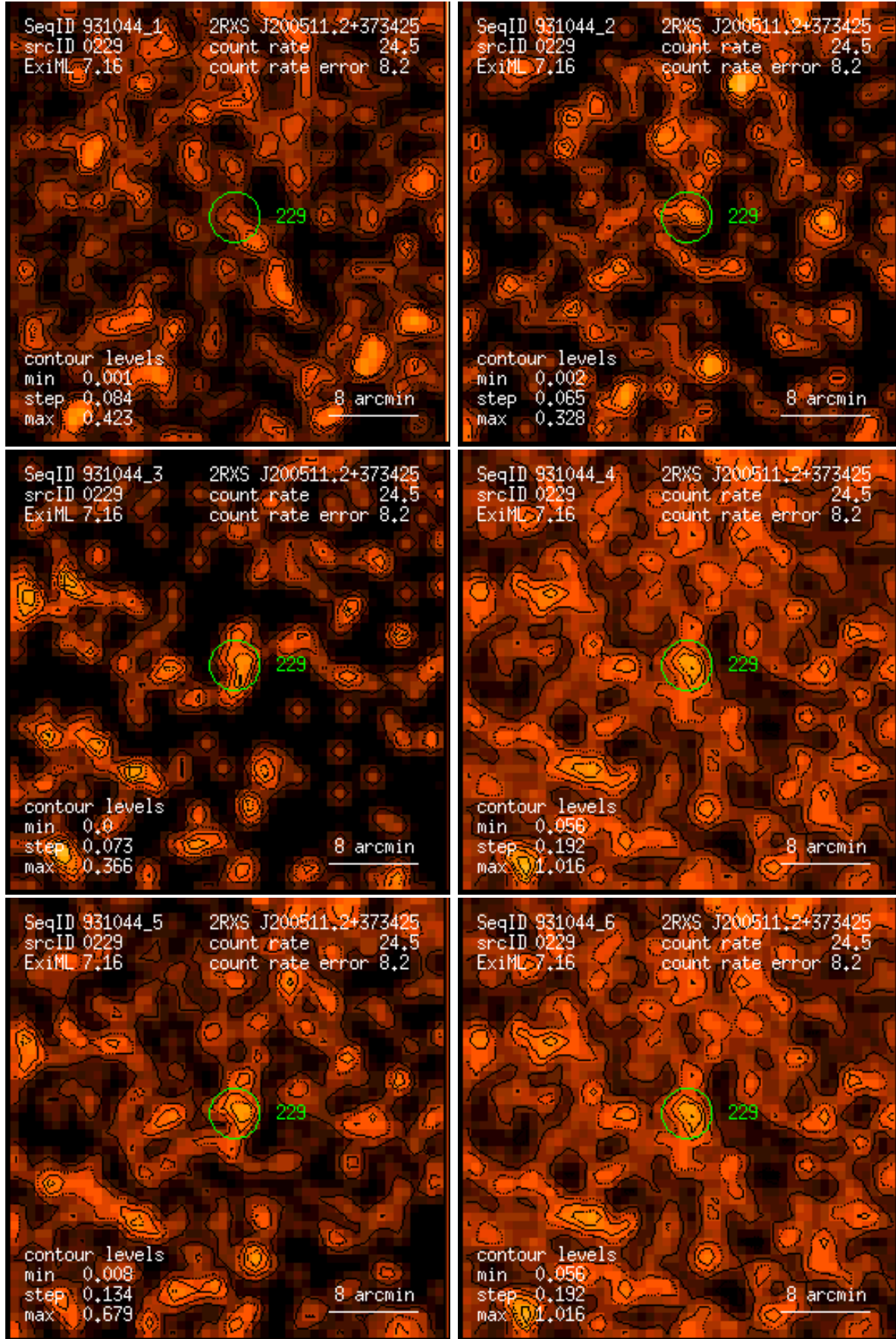
Figure 229: RASS 931044: detection 0229: band rate images, Gaussian filter: (1) PSPC channels 11 – 41, (2) 52 – 90, (3) 91 – 201, (4) 11 – 235, (5) 52 – 201, (6) 11 – 201. Broad band rates in counts/ks. Band rate contour levels in counts/ks/arcmin 2 .
