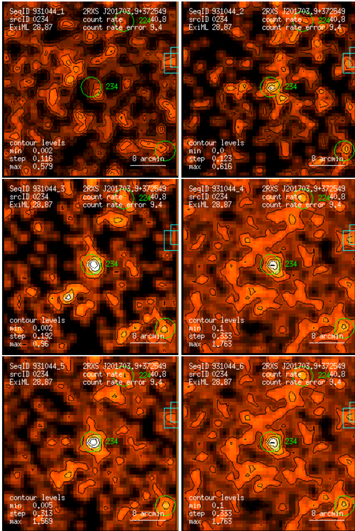
Figure 234: RASS 931044: detection 0234: band rate images, Gaussian filter: (1) PSPC channels 11 – 41, (2) 52 – 90, (3) 91 – 201, (4) 11 – 235, (5) 52 – 201, (6) 11 – 201. Broad band rates in counts/ks. Band rate contour levels in counts/ks/arcmin 2 .
