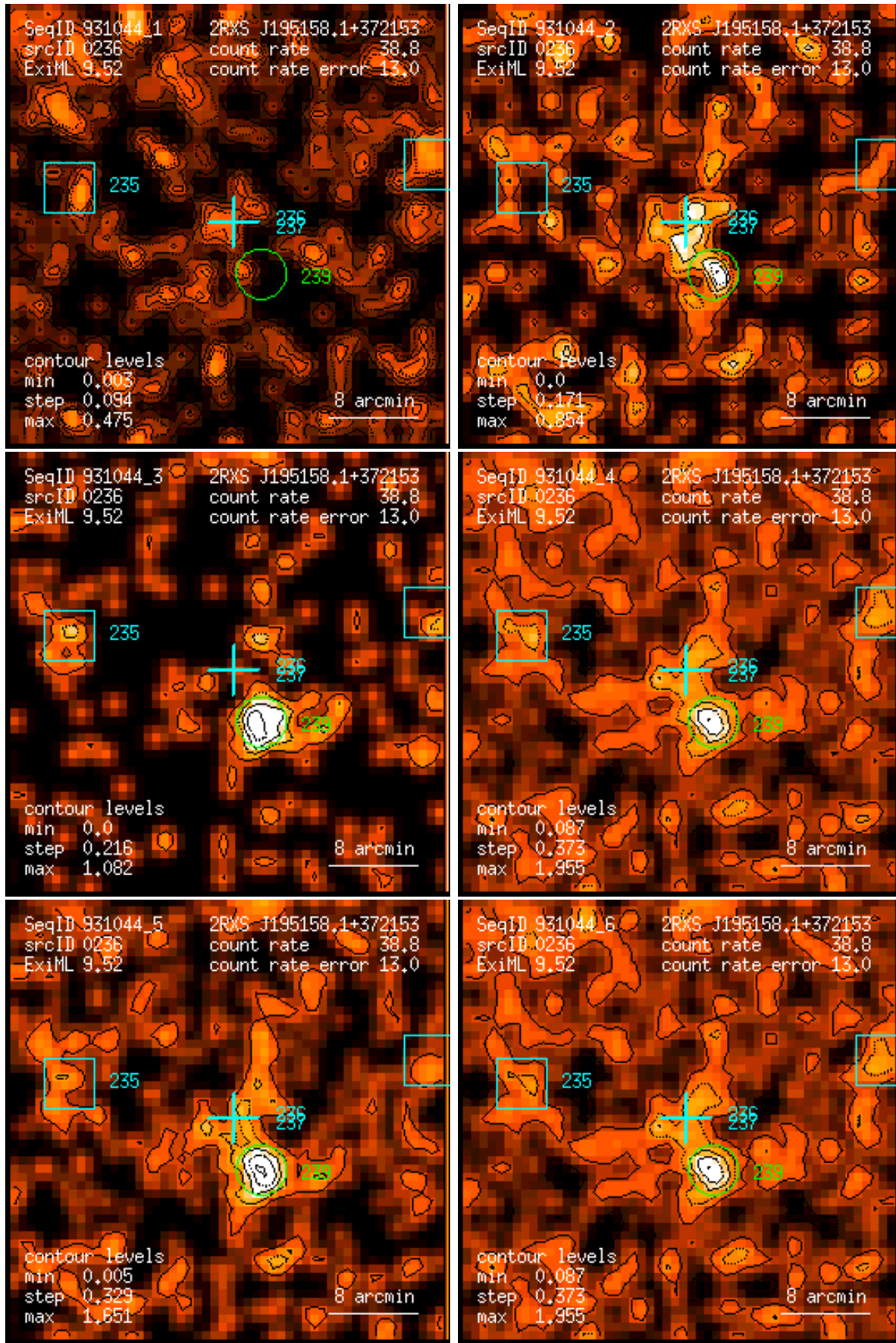
Figure 236: RASS 931044: detection 0236: band rate images, Gaussian filter: (1) PSPC channels 11 – 41, (2) 52 – 90, (3) 91 – 201, (4) 11 – 235, (5) 52 – 201, (6) 11 – 201. Broad band rates in counts/ks. Band rate contour levels in counts/ks/arcmin 2 .
