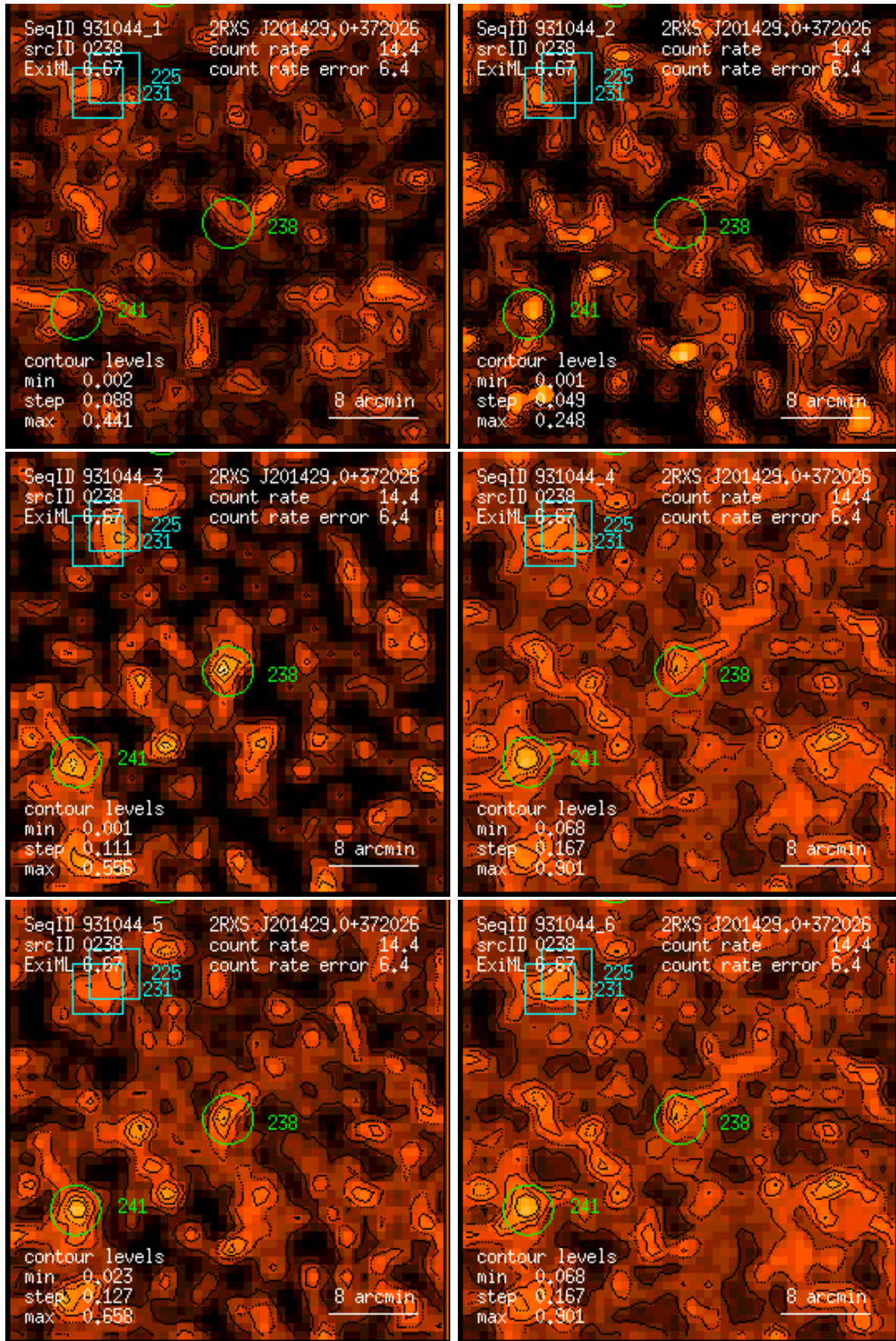
Figure 238: RASS 931044: detection 0238: band rate images, Gaussian filter: (1) PSPC channels 11 – 41, (2) 52 – 90, (3) 91 – 201, (4) 11 – 235, (5) 52 – 201, (6) 11 – 201. Broad band rates in counts/ks. Band rate contour levels in counts/ks/arcmin 2 .
