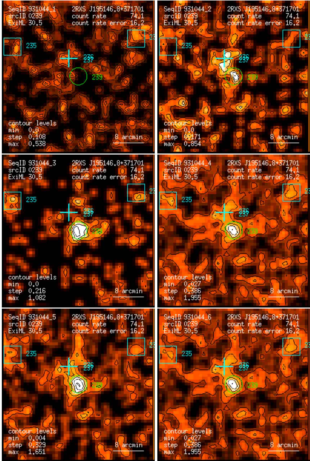
Figure 239: RASS 931044: detection 0239: band rate images, Gaussian filter: (1) PSPC channels 11 – 41, (2) 52 – 90, (3) 91 – 201, (4) 11 – 235, (5) 52 – 201, (6) 11 – 201. Broad band rates in counts/ks. Band rate contour levels in counts/ks/arcmin 2 .
