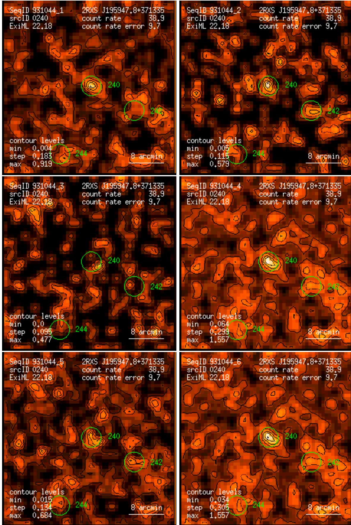
Figure 240: RASS 931044: detection 0240: band rate images, Gaussian filter: (1) PSPC channels 11 – 41, (2) 52 – 90, (3) 91 – 201, (4) 11 – 235, (5) 52 – 201, (6) 11 – 201. Broad band rates in counts/ks. Band rate contour levels in counts/ks/arcmin 2 .
