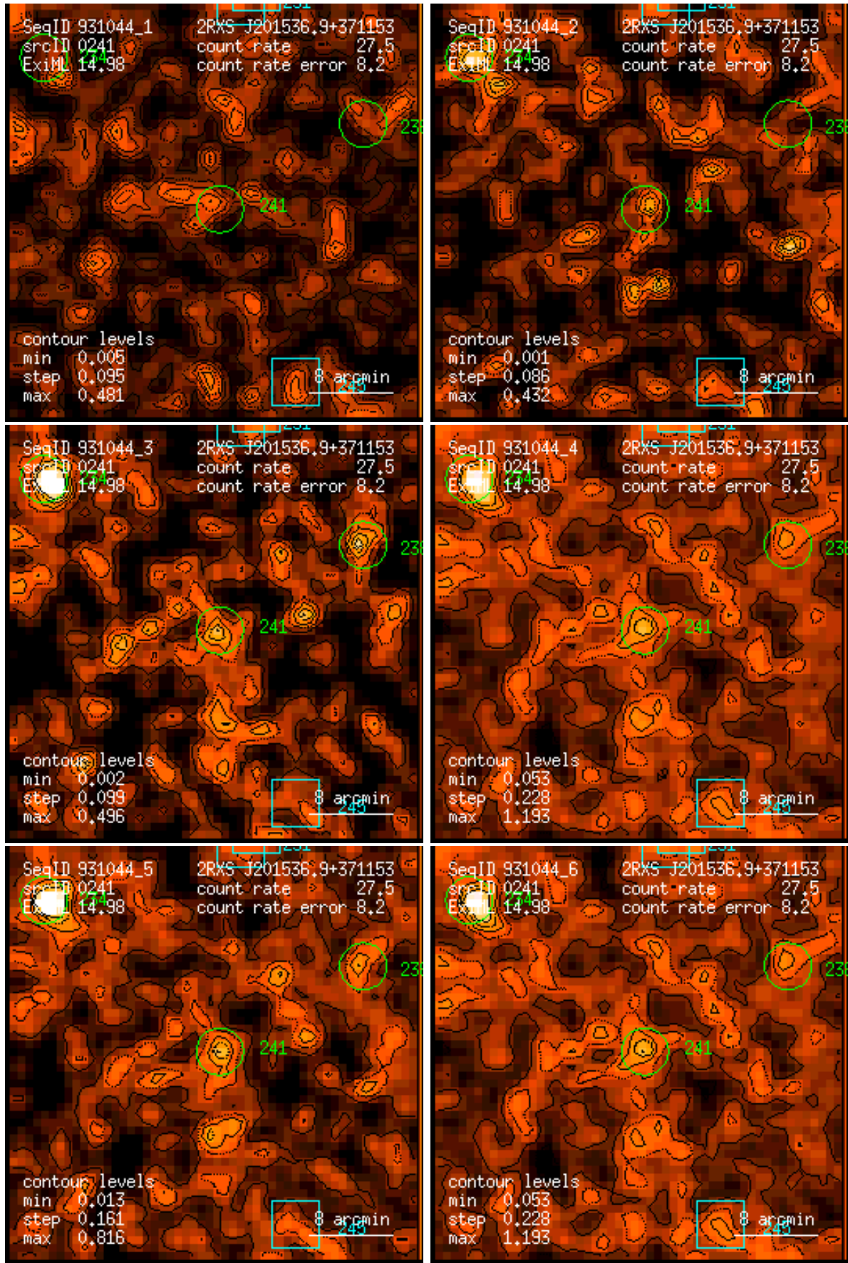
Figure 241: RASS 931044: detection 0241: band rate images, Gaussian filter: (1) PSPC channels 11 – 41, (2) 52 – 90, (3) 91 – 201, (4) 11 – 235, (5) 52 – 201, (6) 11 – 201. Broad band rates in counts/ks. Band rate contour levels in counts/ks/arcmin 2 .
