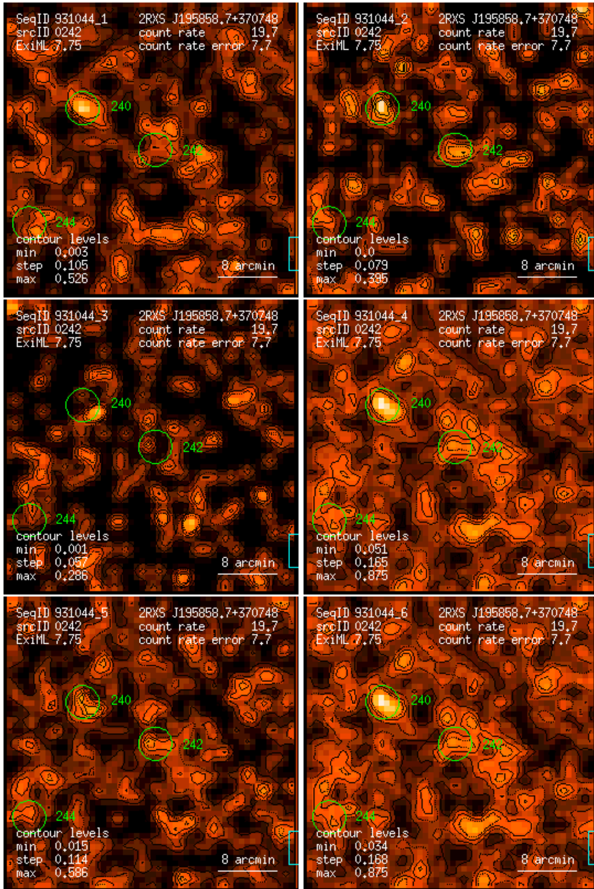
Figure 242: RASS 931044: detection 0242: band rate images, Gaussian filter: (1) PSPC channels 11 – 41, (2) 52 – 90, (3) 91 – 201, (4) 11 – 235, (5) 52 – 201, (6) 11 – 201. Broad band rates in counts/ks. Band rate contour levels in counts/ks/arcmin 2 .
