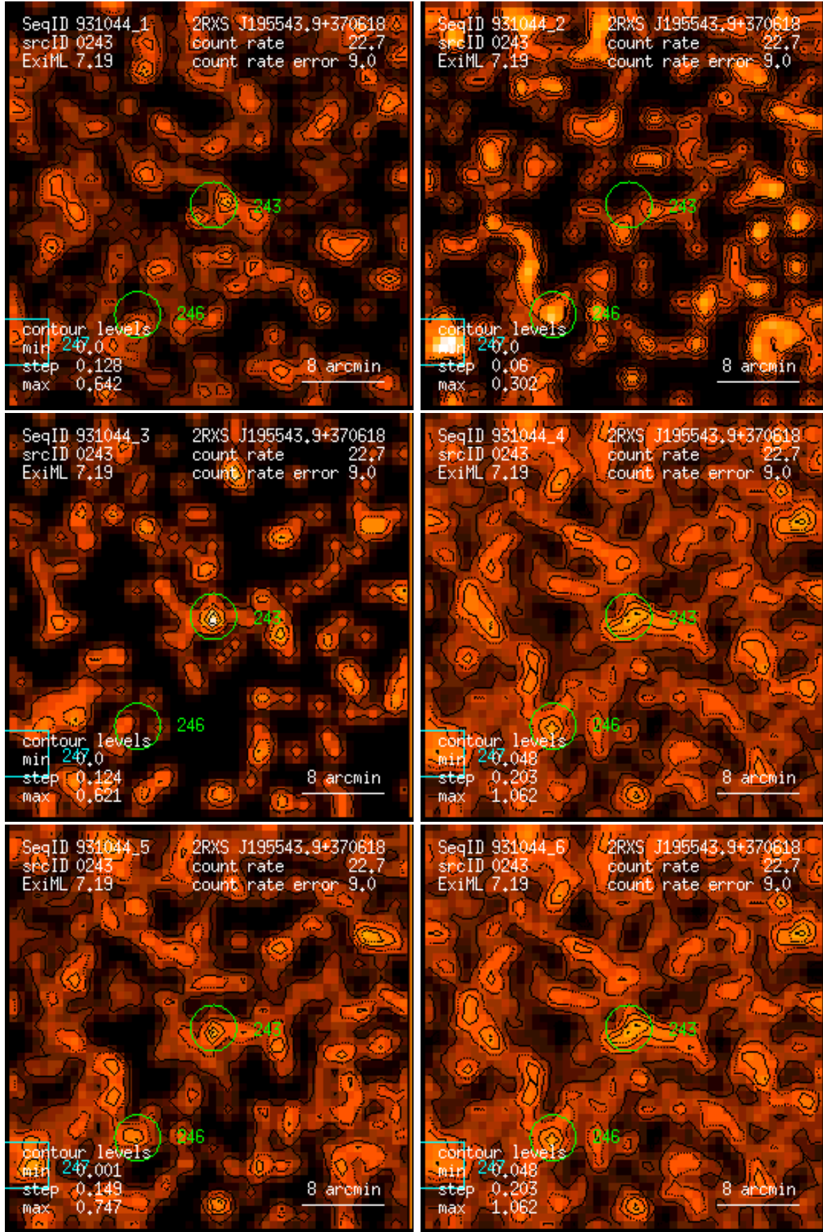
Figure 243: RASS 931044: detection 0243: band rate images, Gaussian filter: (1) PSPC channels 11 – 41, (2) 52 – 90, (3) 91 – 201, (4) 11 – 235, (5) 52 – 201, (6) 11 – 201. Broad band rates in counts/ks. Band rate contour levels in counts/ks/arcmin 2 .
