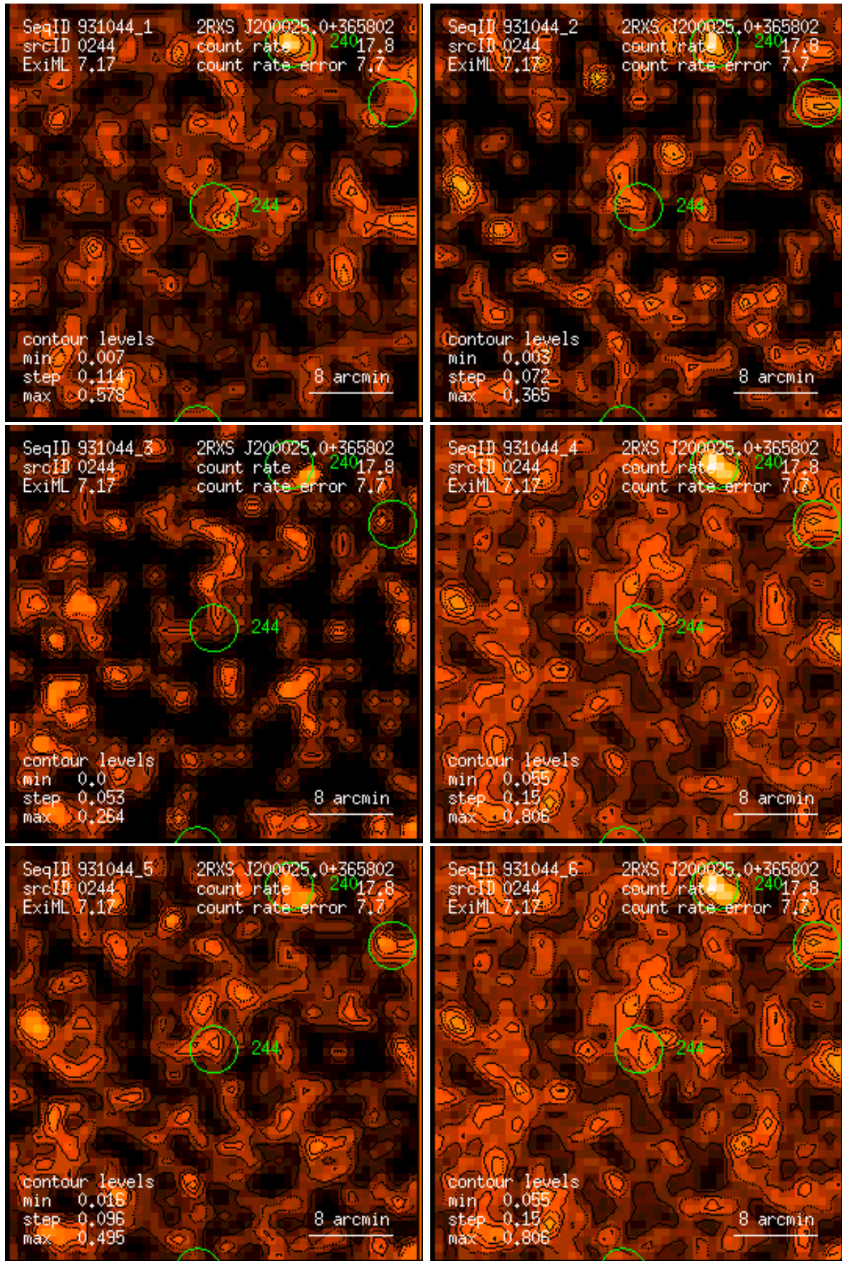
Figure 244: RASS 931044: detection 0244: band rate images, Gaussian filter: (1) PSPC channels 11 – 41, (2) 52 – 90, (3) 91 – 201, (4) 11 – 235, (5) 52 – 201, (6) 11 – 201. Broad band rates in counts/ks. Band rate contour levels in counts/ks/arcmin 2 .
