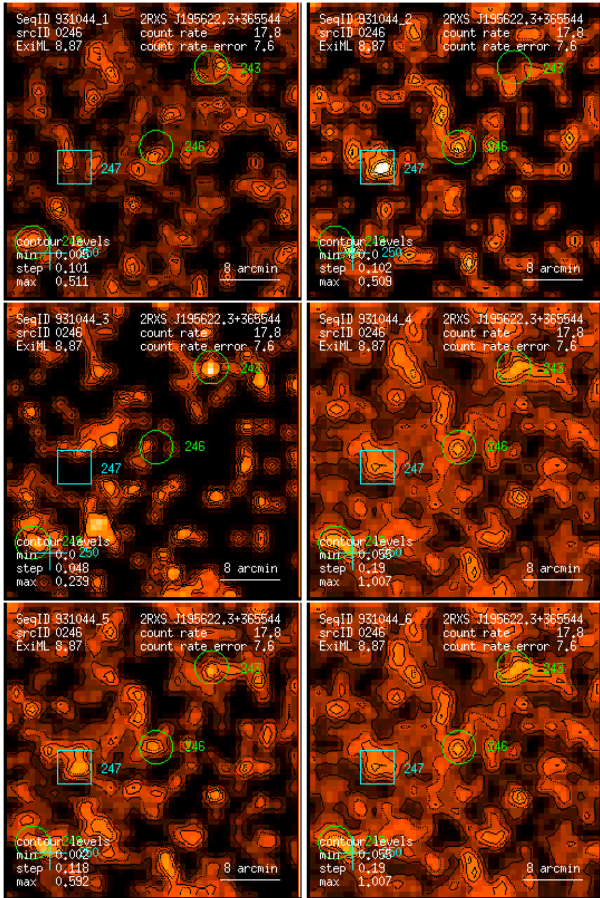
Figure 246: RASS 931044: detection 0246: band rate images, Gaussian filter: (1) PSPC channels 11 – 41, (2) 52 – 90, (3) 91 – 201, (4) 11 – 235, (5) 52 – 201, (6) 11 – 201. Broad band rates in counts/ks. Band rate contour levels in counts/ks/arcmin 2 .
