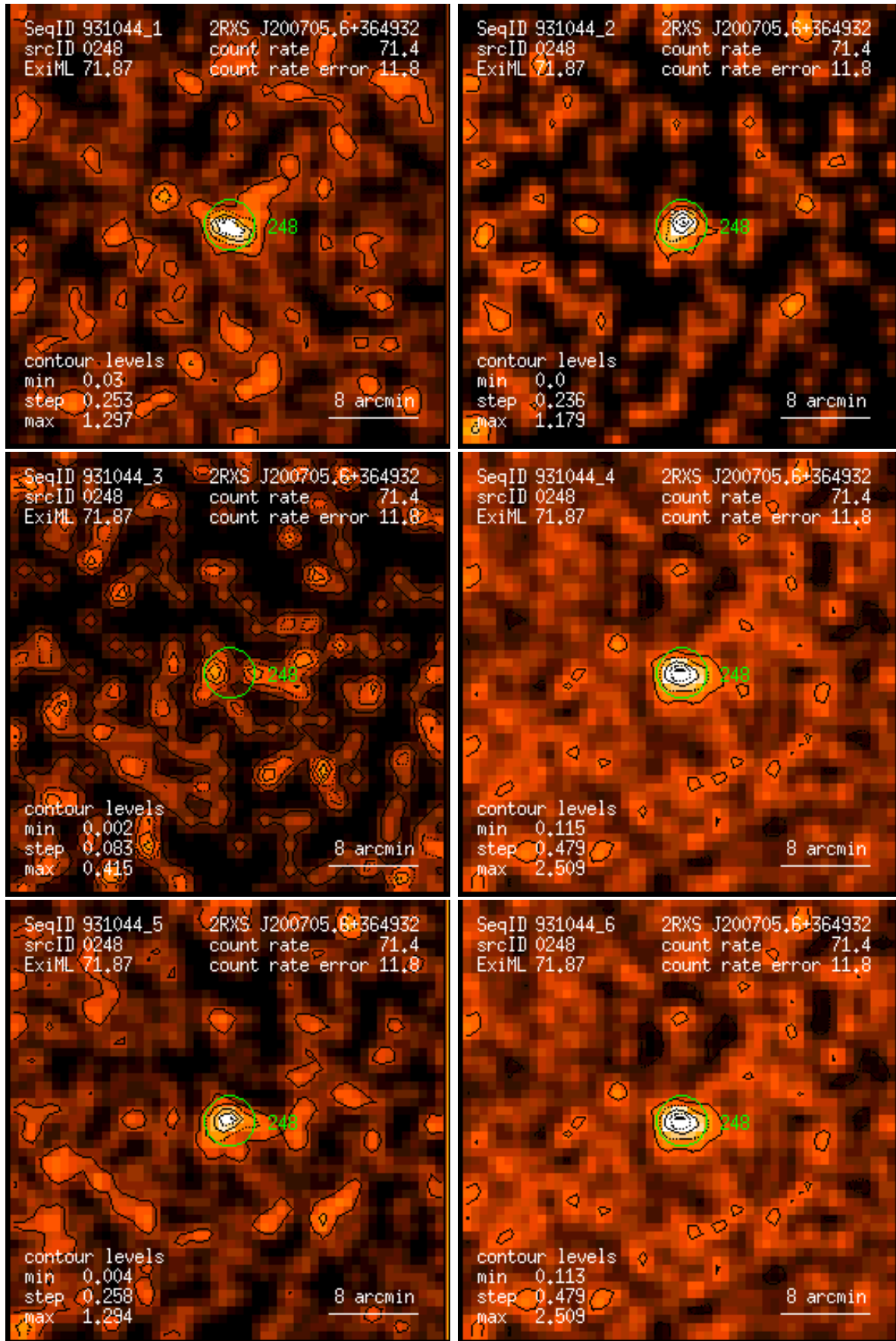
Figure 248: RASS 931044: detection 0248: band rate images, Gaussian filter: (1) PSPC channels 11 – 41, (2) 52 – 90, (3) 91 – 201, (4) 11 – 235, (5) 52 – 201, (6) 11 – 201. Broad band rates in counts/ks. Band rate contour levels in counts/ks/arcmin 2 .
