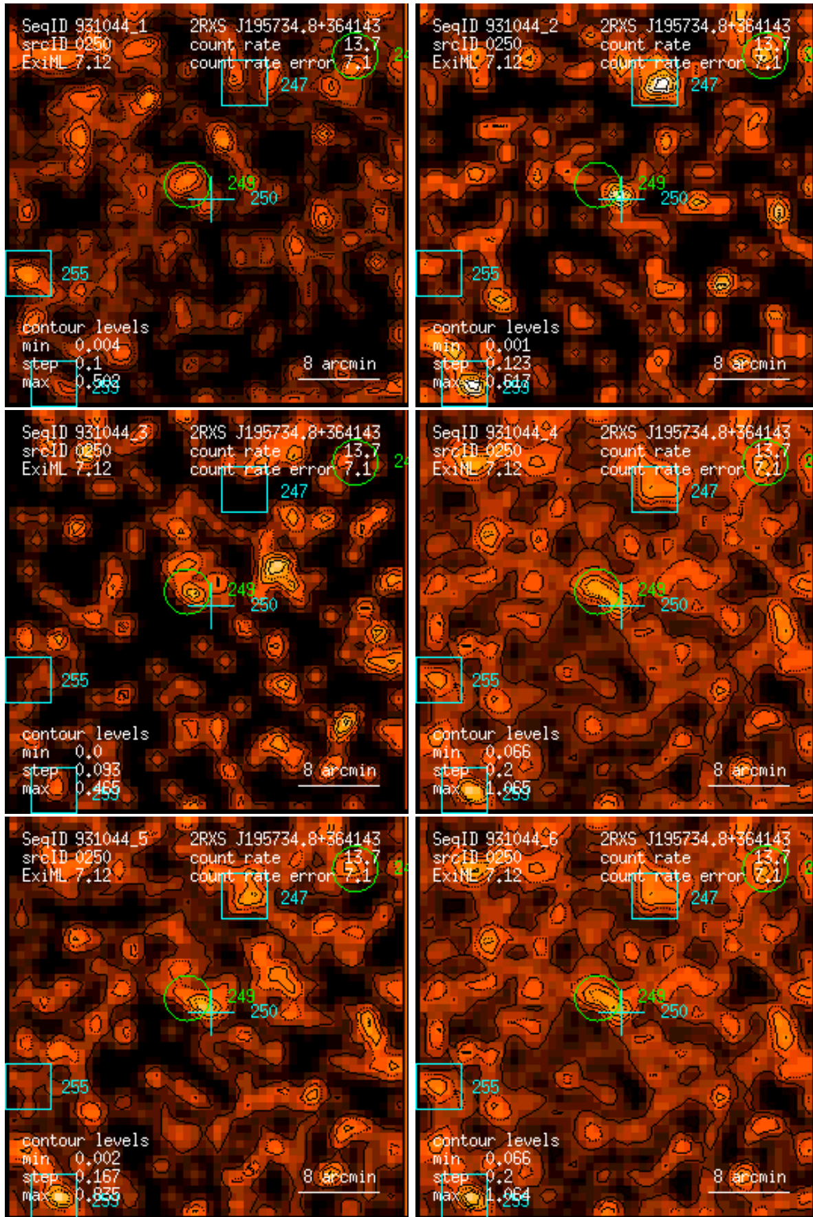
Figure 250: RASS 931044: detection 0250: band rate images, Gaussian filter: (1) PSPC channels 11 – 41, (2) 52 – 90, (3) 91 – 201, (4) 11 – 235, (5) 52 – 201, (6) 11 – 201. Broad band rates in counts/ks. Band rate contour levels in counts/ks/arcmin 2 .
