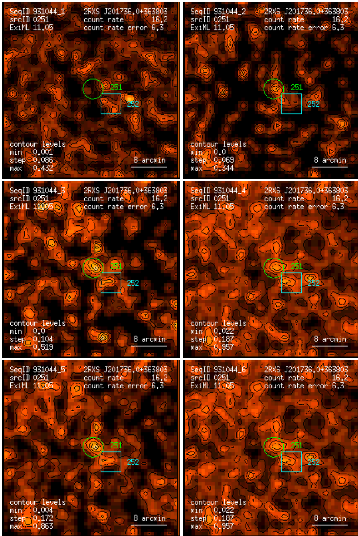
Figure 251: RASS 931044: detection 0251: band rate images, Gaussian filter: (1) PSPC channels 11 – 41, (2) 52 – 90, (3) 91 – 201, (4) 11 – 235, (5) 52 – 201, (6) 11 – 201. Broad band rates in counts/ks. Band rate contour levels in counts/ks/arcmin 2 .
