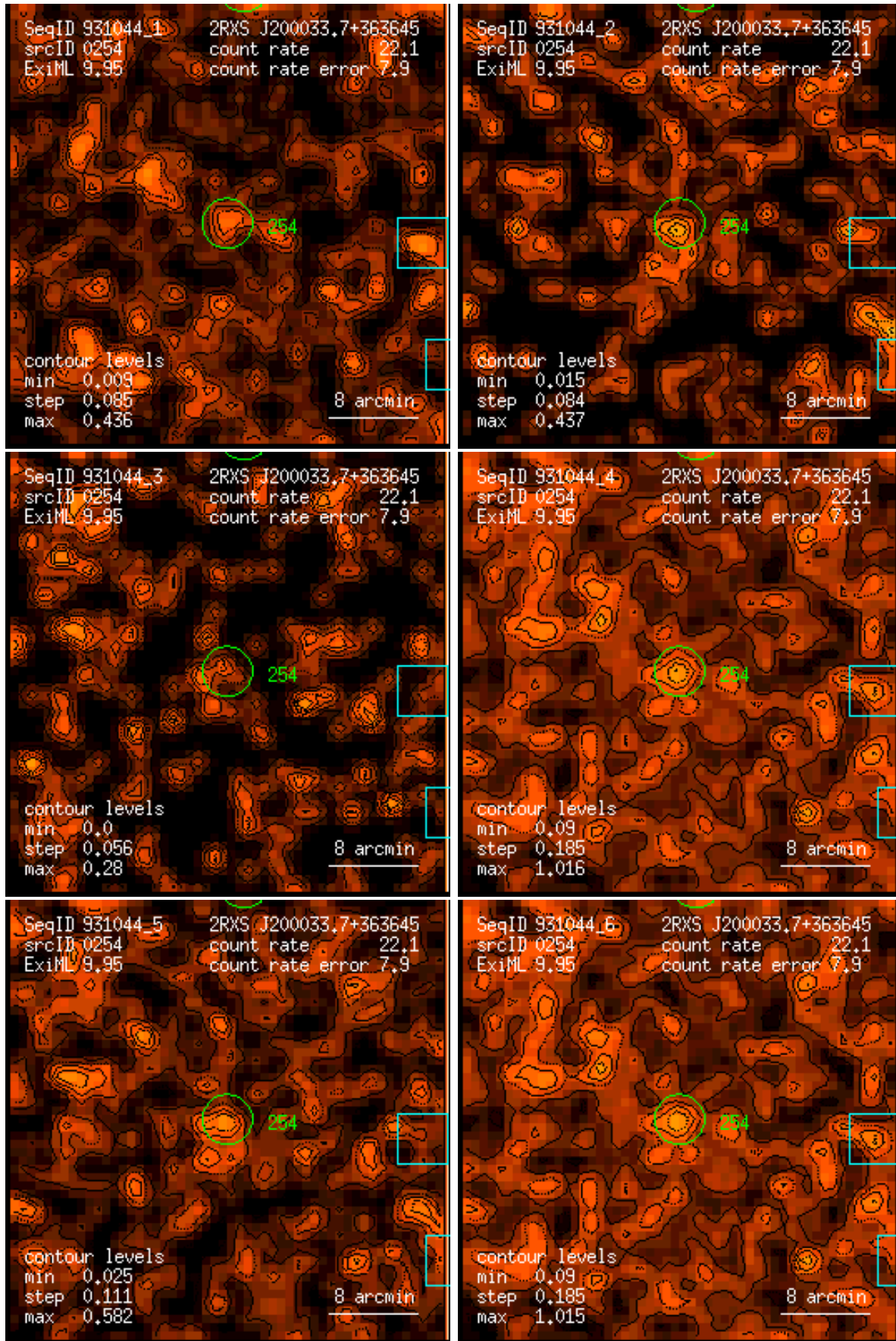
Figure 254: RASS 931044: detection 0254: band rate images, Gaussian filter: (1) PSPC channels 11 – 41, (2) 52 – 90, (3) 91 – 201, (4) 11 – 235, (5) 52 – 201, (6) 11 – 201. Broad band rates in counts/ks. Band rate contour levels in counts/ks/arcmin 2 .
