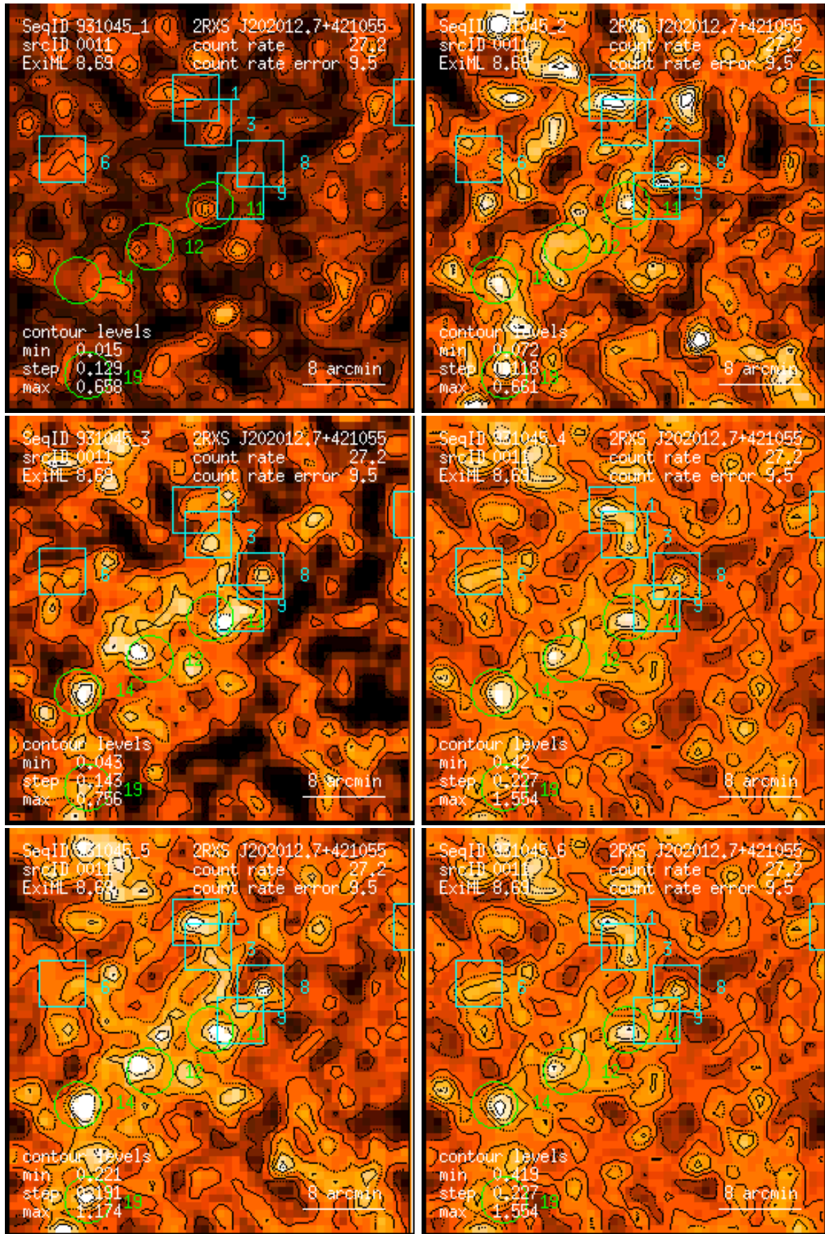
Figure 11: RASS 931045: detection 0011: band rate images, Gaussian filter: (1) PSPC channels 11 – 41, (2) 52 – 90, (3) 91 – 201, (4) 11 – 235, (5) 52 – 201, (6) 11 – 201. Broad band rates in counts/ks. Band rate contour levels in counts/ks/arcmin 2 .
