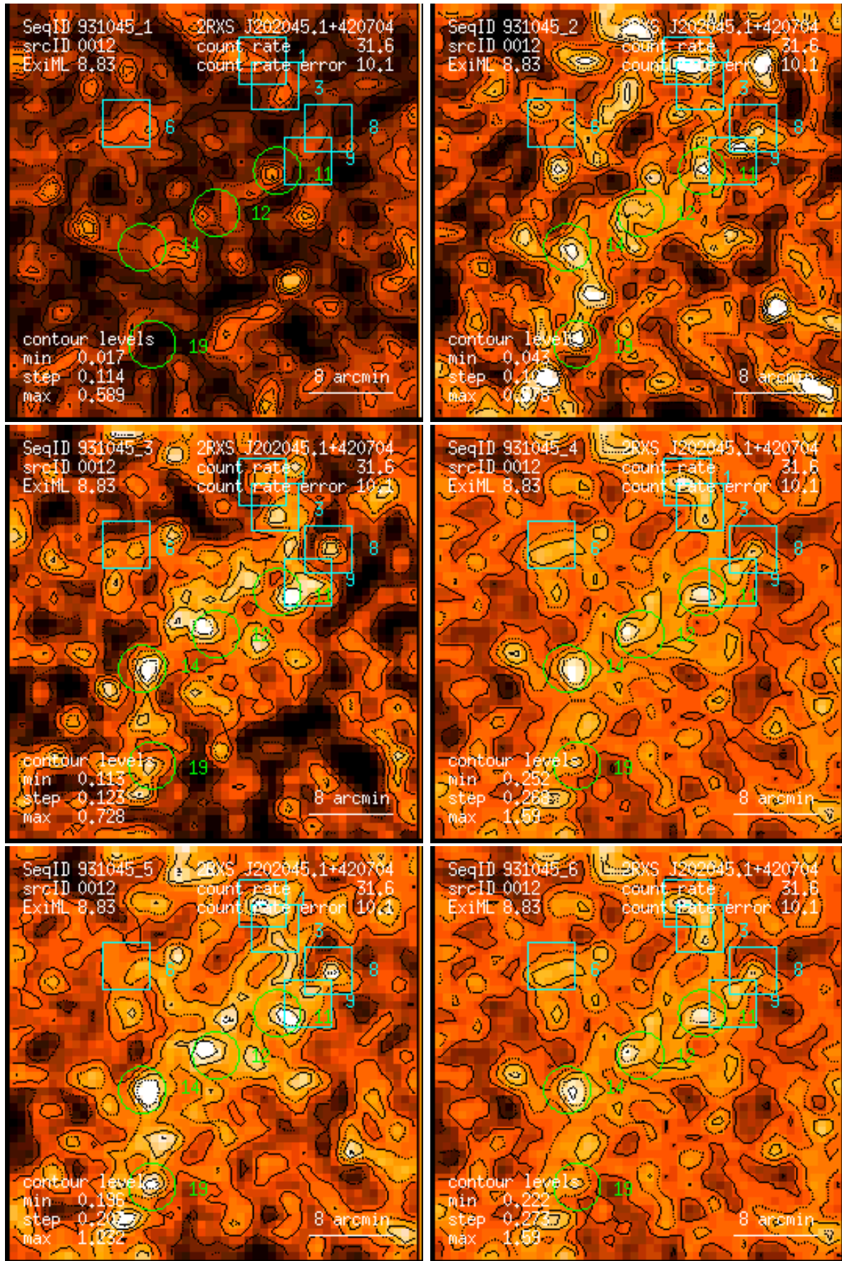
Figure 12: RASS 931045: detection 0012: band rate images, Gaussian filter: (1) PSPC channels 11 – 41, (2) 52 – 90, (3) 91 – 201, (4) 11 – 235, (5) 52 – 201, (6) 11 – 201. Broad band rates in counts/ks. Band rate contour levels in counts/ks/arcmin 2 .
