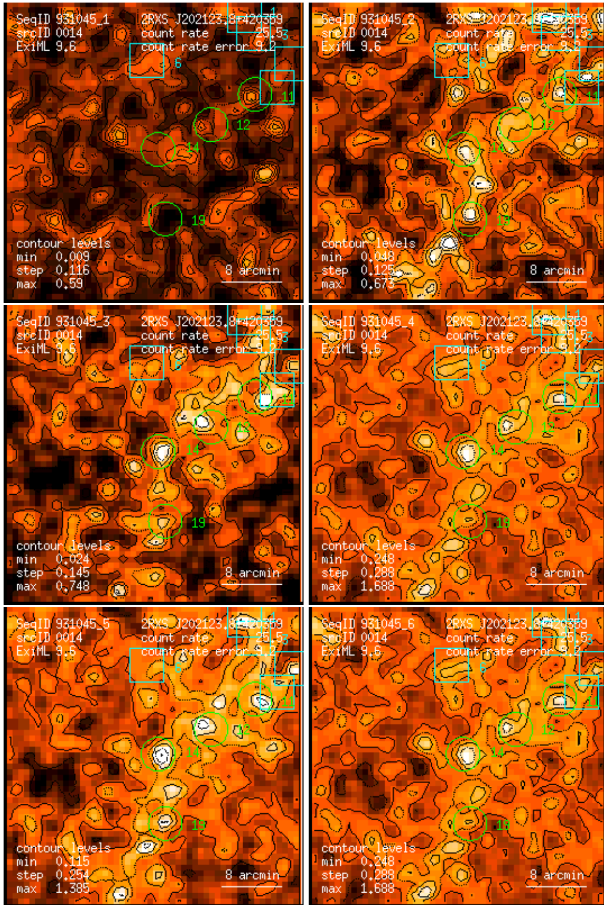
Figure 14: RASS 931045: detection 0014: band rate images, Gaussian filter: (1) PSPC channels 11 – 41, (2) 52 – 90, (3) 91 – 201, (4) 11 – 235, (5) 52 – 201, (6) 11 – 201. Broad band rates in counts/ks. Band rate contour levels in counts/ks/arcmin 2 .
