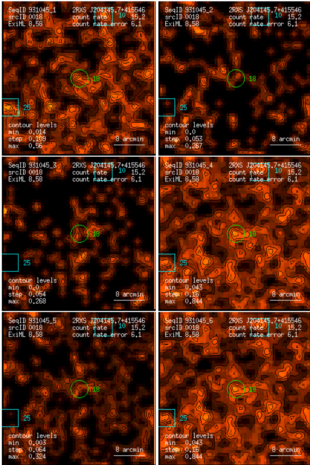
Figure 18: RASS 931045: detection 0018: band rate images, Gaussian filter: (1) PSPC channels 11 – 41, (2) 52 – 90, (3) 91 – 201, (4) 11 – 235, (5) 52 – 201, (6) 11 – 201. Broad band rates in counts/ks. Band rate contour levels in counts/ks/arcmin 2 .
