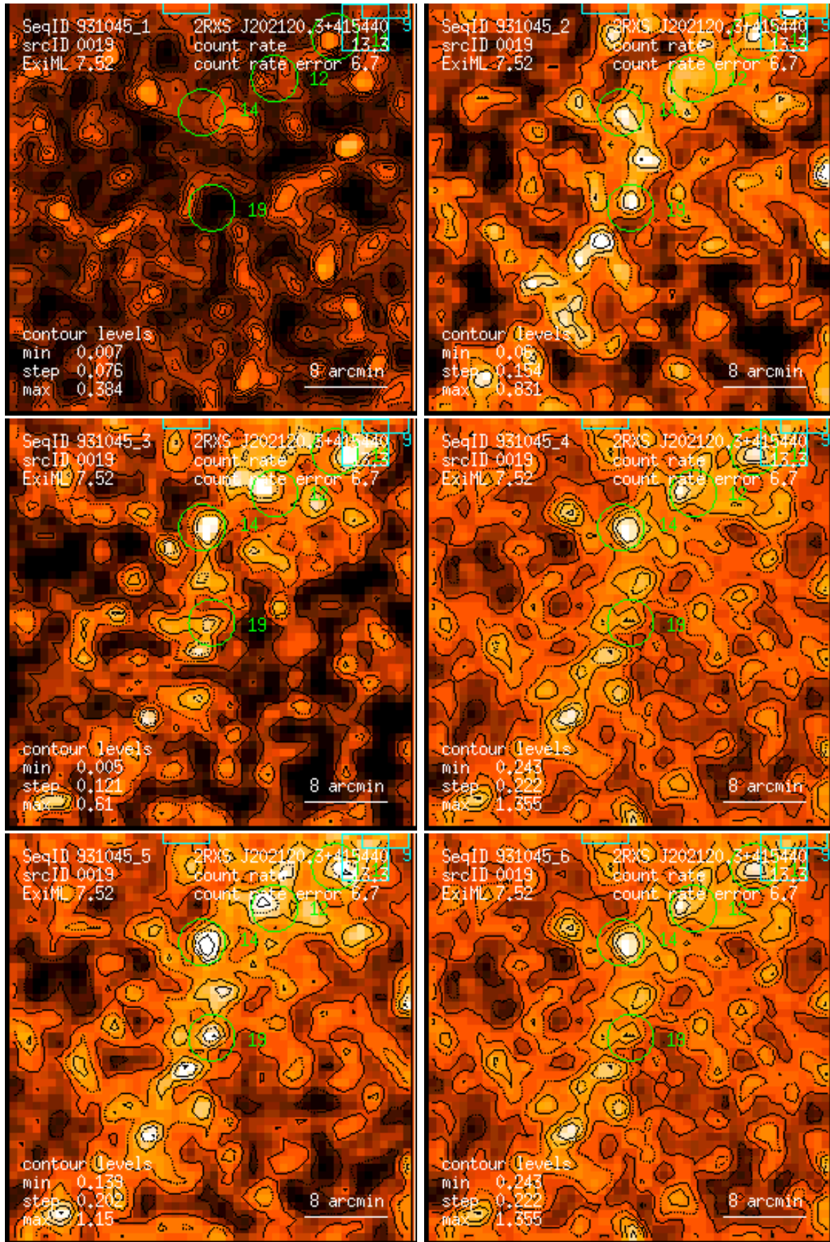
Figure 19: RASS 931045: detection 0019: band rate images, Gaussian filter: (1) PSPC channels 11 – 41, (2) 52 – 90, (3) 91 – 201, (4) 11 – 235, (5) 52 – 201, (6) 11 – 201. Broad band rates in counts/ks. Band rate contour levels in counts/ks/arcmin 2 .
