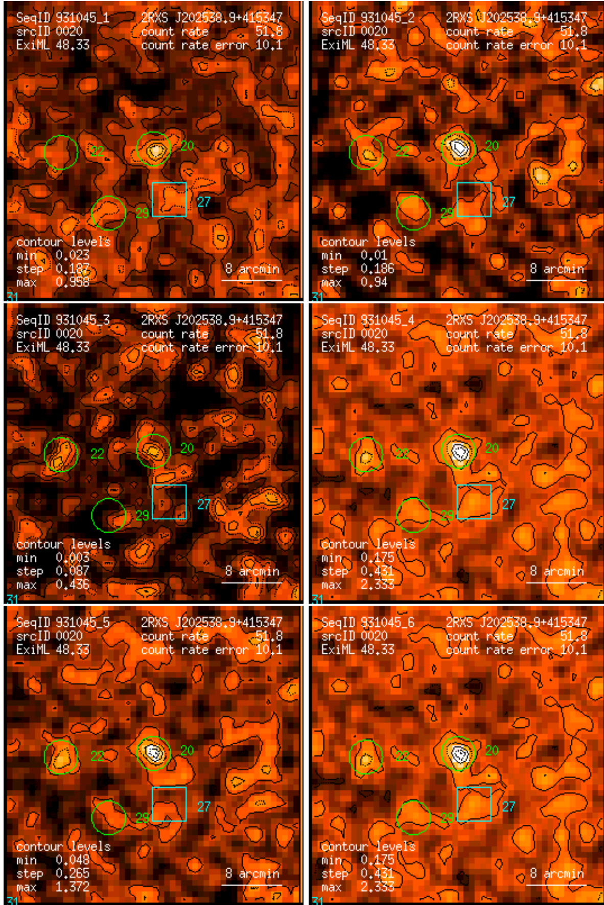
Figure 20: RASS 931045: detection 0020: band rate images, Gaussian filter: (1) PSPC channels 11 – 41, (2) 52 – 90, (3) 91 – 201, (4) 11 – 235, (5) 52 – 201, (6) 11 – 201. Broad band rates in counts/ks. Band rate contour levels in counts/ks/arcmin 2 .
