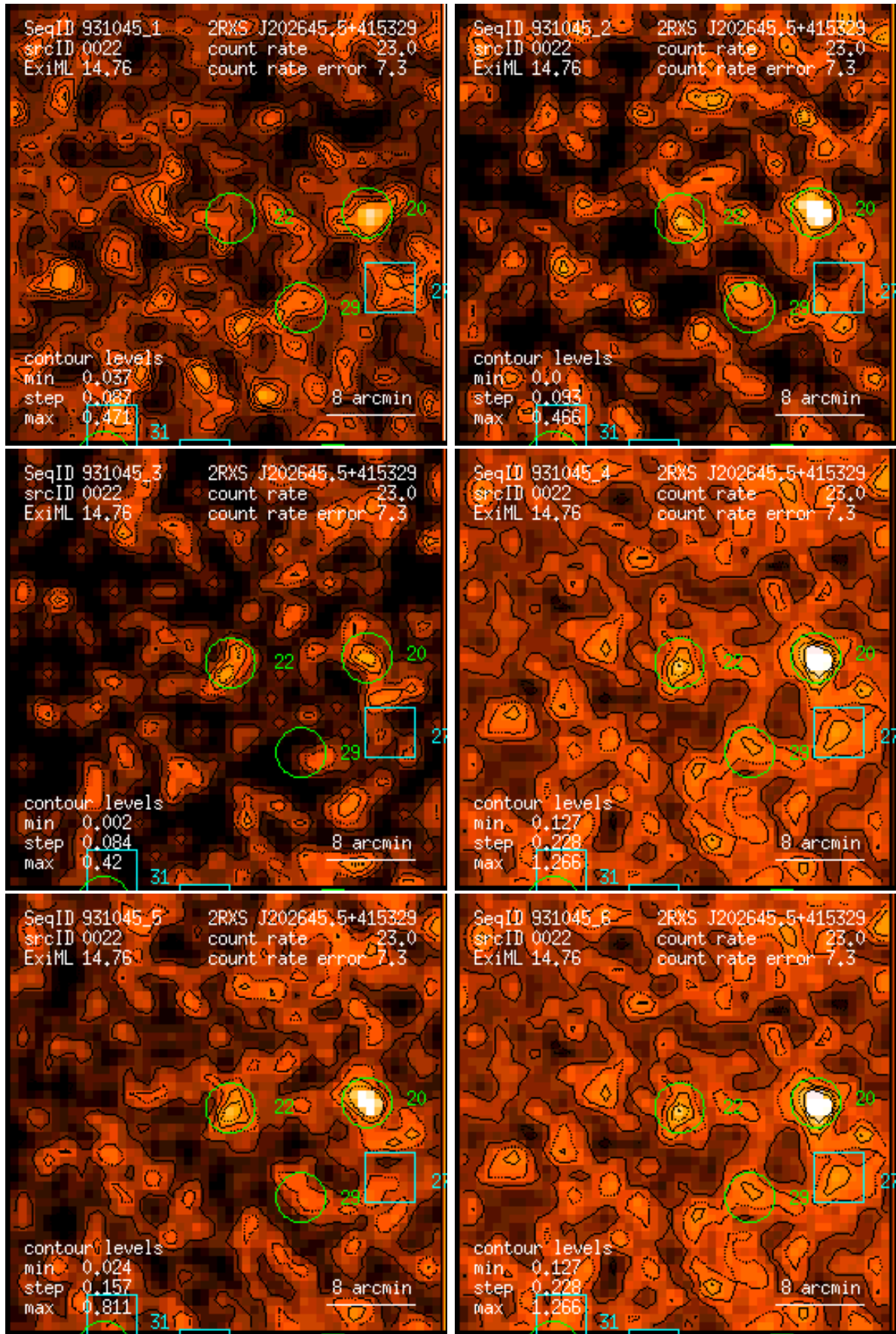
Figure 22: RASS 931045: detection 0022: band rate images, Gaussian filter: (1) PSPC channels 11 – 41, (2) 52 – 90, (3) 91 – 201, (4) 11 – 235, (5) 52 – 201, (6) 11 – 201. Broad band rates in counts/ks. Band rate contour levels in counts/ks/arcmin 2 .
