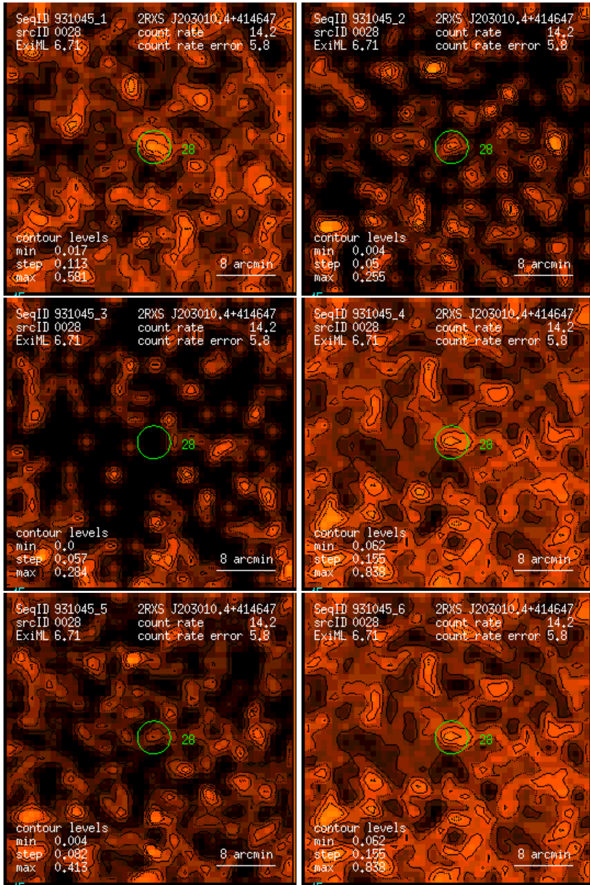
Figure 28: RASS 931045: detection 0028: band rate images, Gaussian filter: (1) PSPC channels 11 – 41, (2) 52 – 90, (3) 91 – 201, (4) 11 – 235, (5) 52 – 201, (6) 11 – 201. Broad band rates in counts/ks. Band rate contour levels in counts/ks/arcmin 2 .
