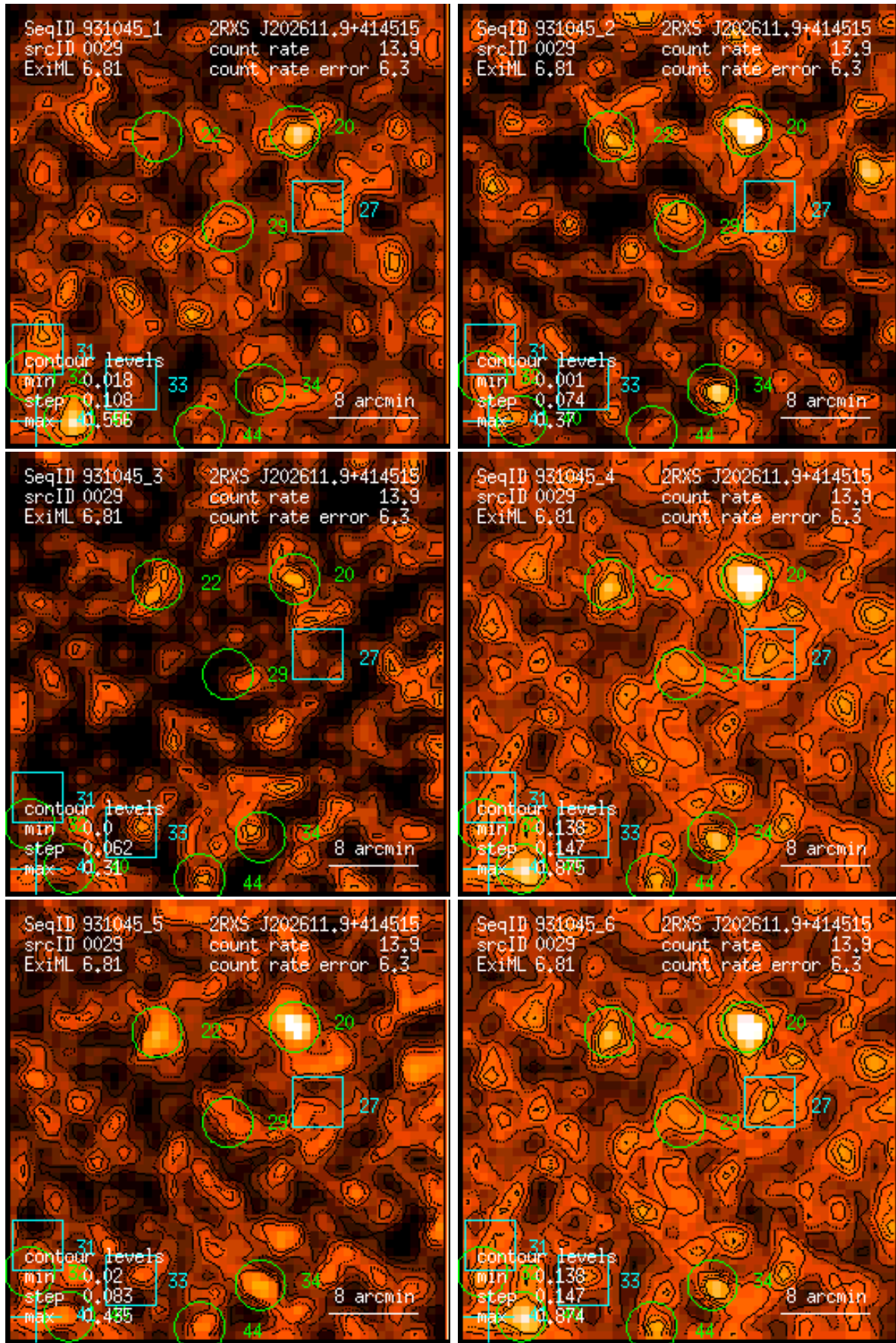
Figure 29: RASS 931045: detection 0029: band rate images, Gaussian filter: (1) PSPC channels 11 – 41, (2) 52 – 90, (3) 91 – 201, (4) 11 – 235, (5) 52 – 201, (6) 11 – 201. Broad band rates in counts/ks. Band rate contour levels in counts/ks/arcmin 2 .
