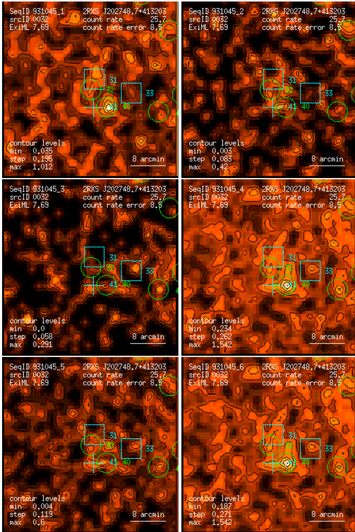
Figure 32: RASS 931045: detection 0032: band rate images, Gaussian filter: (1) PSPC channels 11 – 41, (2) 52 – 90, (3) 91 – 201, (4) 11 – 235, (5) 52 – 201, (6) 11 – 201. Broad band rates in counts/ks. Band rate contour levels in counts/ks/arcmin 2 .
