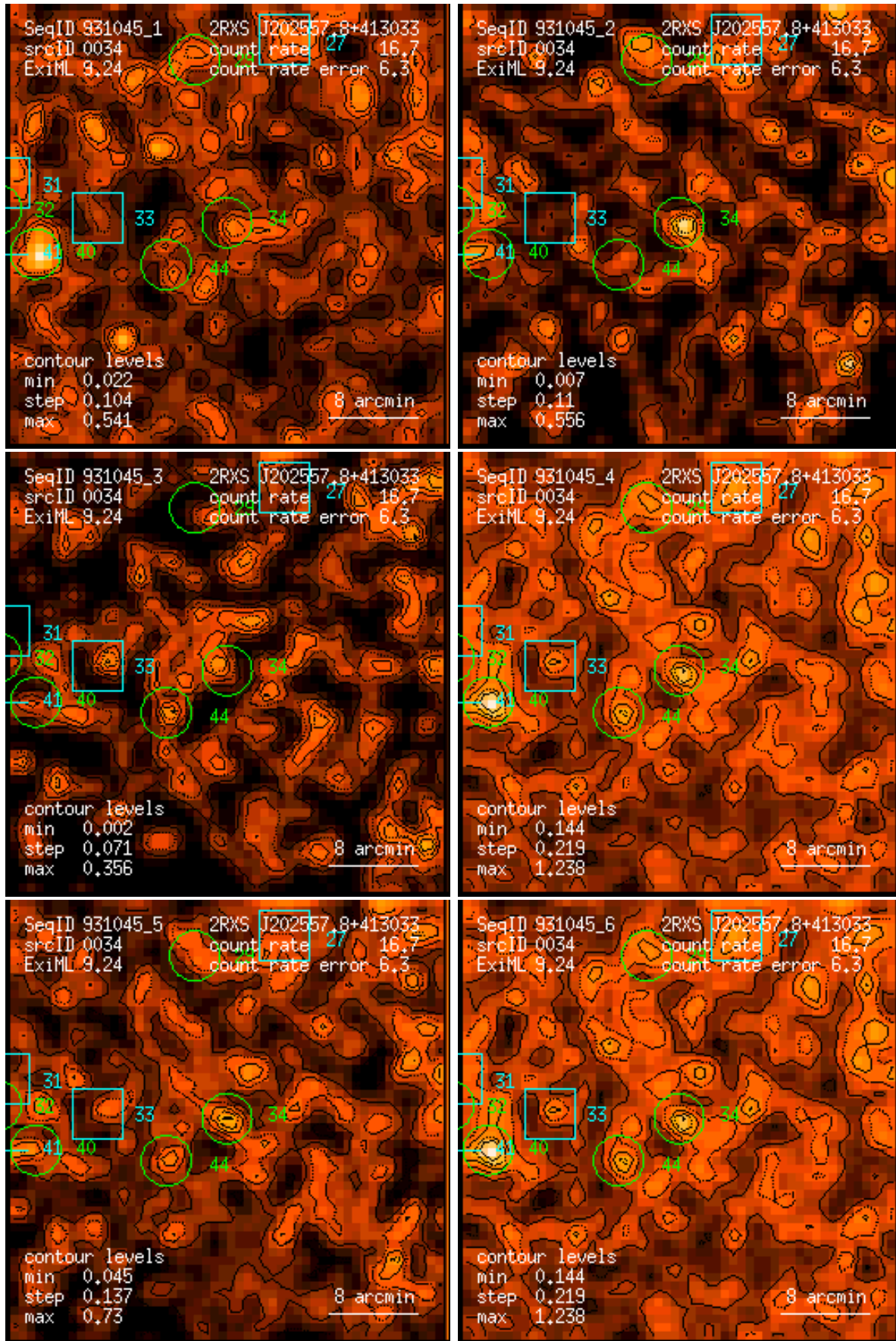
Figure 34: RASS 931045: detection 0034: band rate images, Gaussian filter: (1) PSPC channels 11 – 41, (2) 52 – 90, (3) 91 – 201, (4) 11 – 235, (5) 52 – 201, (6) 11 – 201. Broad band rates in counts/ks. Band rate contour levels in counts/ks/arcmin 2 .
