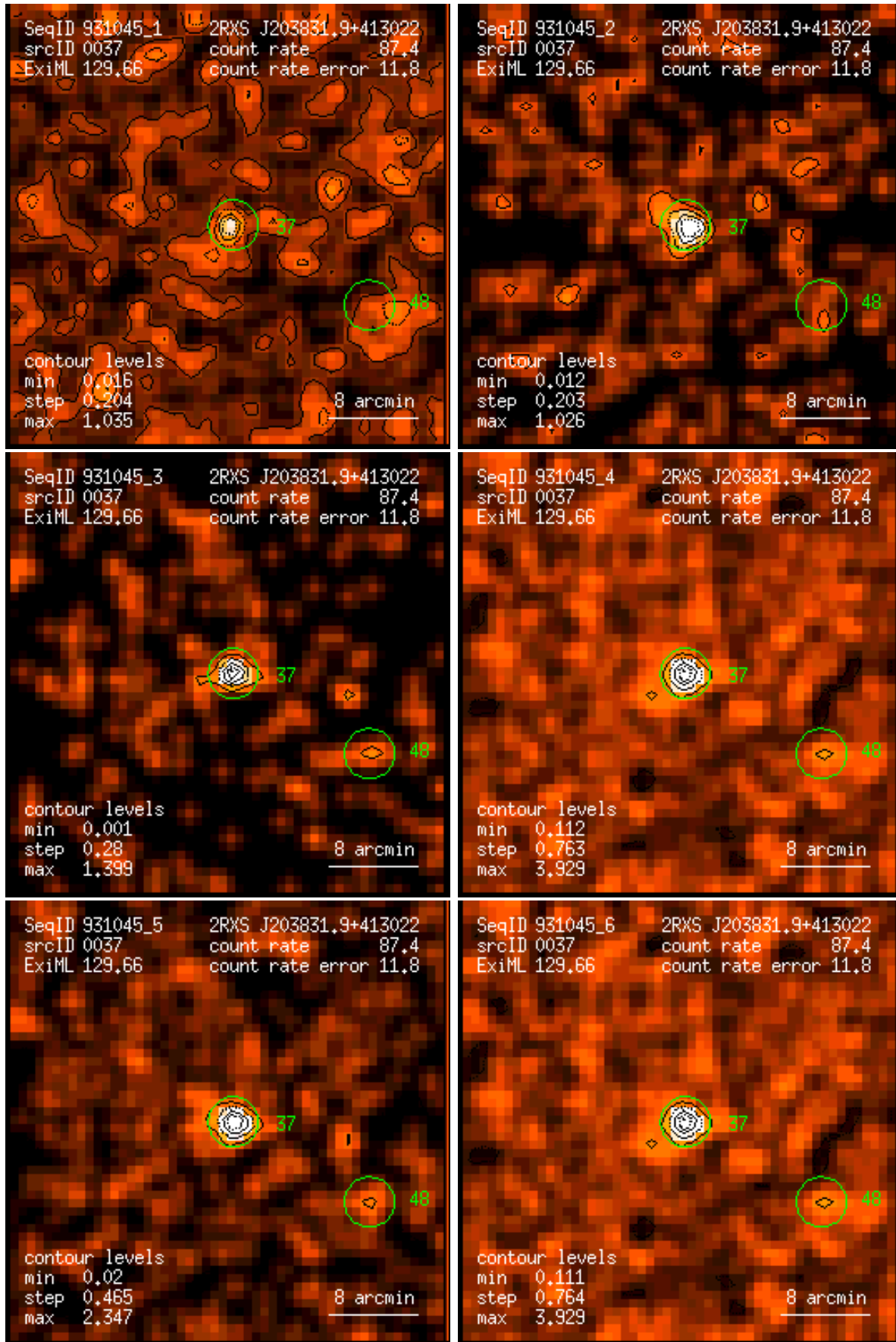
Figure 37: RASS 931045: detection 0037: band rate images, Gaussian filter: (1) PSPC channels 11 – 41, (2) 52 – 90, (3) 91 – 201, (4) 11 – 235, (5) 52 – 201, (6) 11 – 201. Broad band rates in counts/ks. Band rate contour levels in counts/ks/arcmin 2 .
