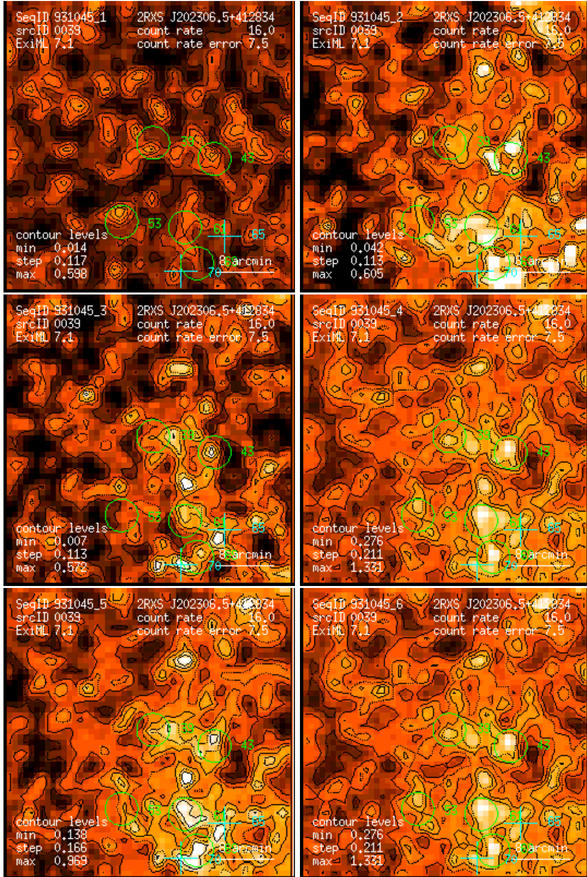
Figure 39: RASS 931045: detection 0039: band rate images, Gaussian filter: (1) PSPC channels 11 – 41, (2) 52 – 90, (3) 91 – 201, (4) 11 – 235, (5) 52 – 201, (6) 11 – 201. Broad band rates in counts/ks. Band rate contour levels in counts/ks/arcmin 2 .
