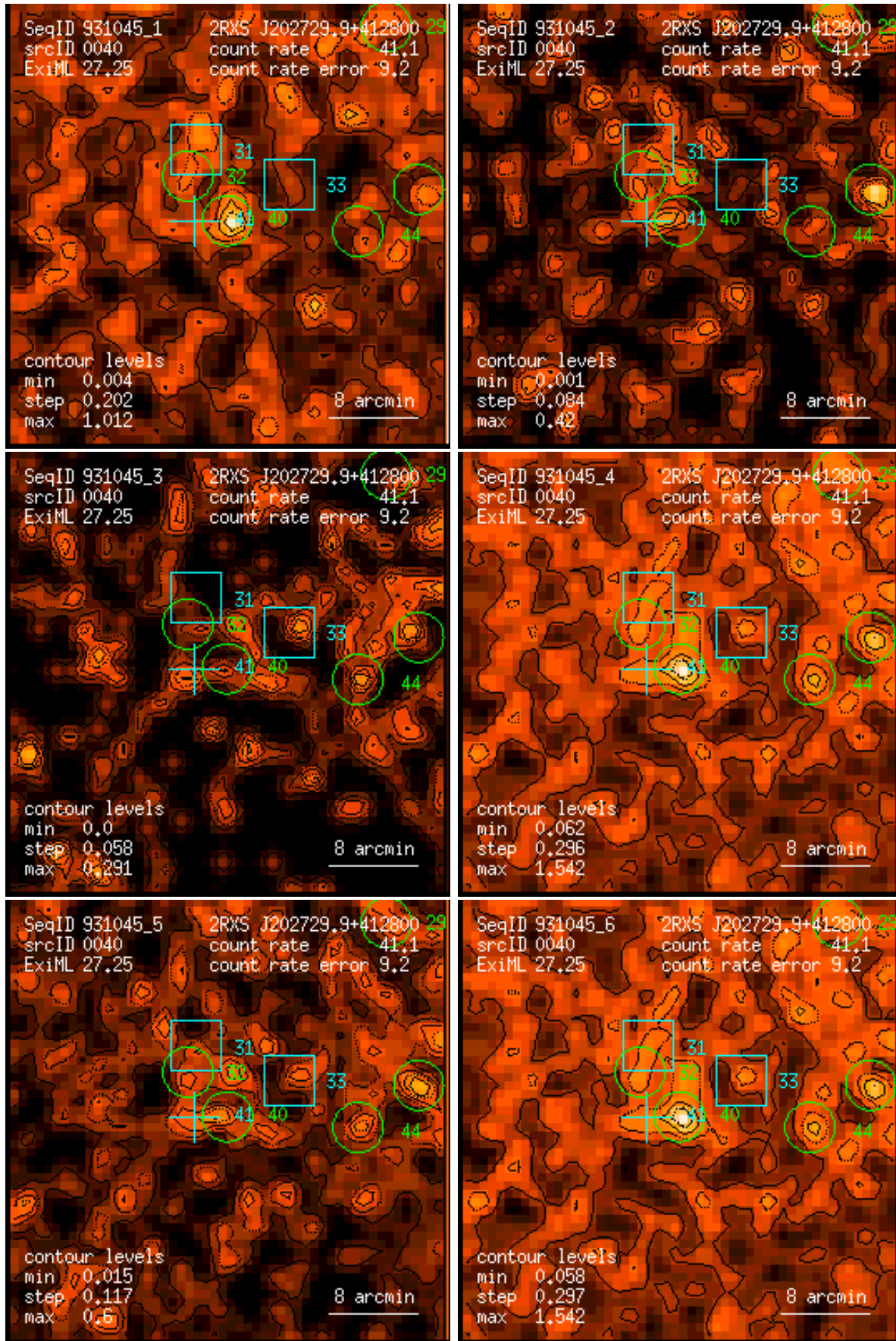
Figure 40: RASS 931045: detection 0040: band rate images, Gaussian filter: (1) PSPC channels 11 – 41, (2) 52 – 90, (3) 91 – 201, (4) 11 – 235, (5) 52 – 201, (6) 11 – 201. Broad band rates in counts/ks. Band rate contour levels in counts/ks/arcmin 2 .
