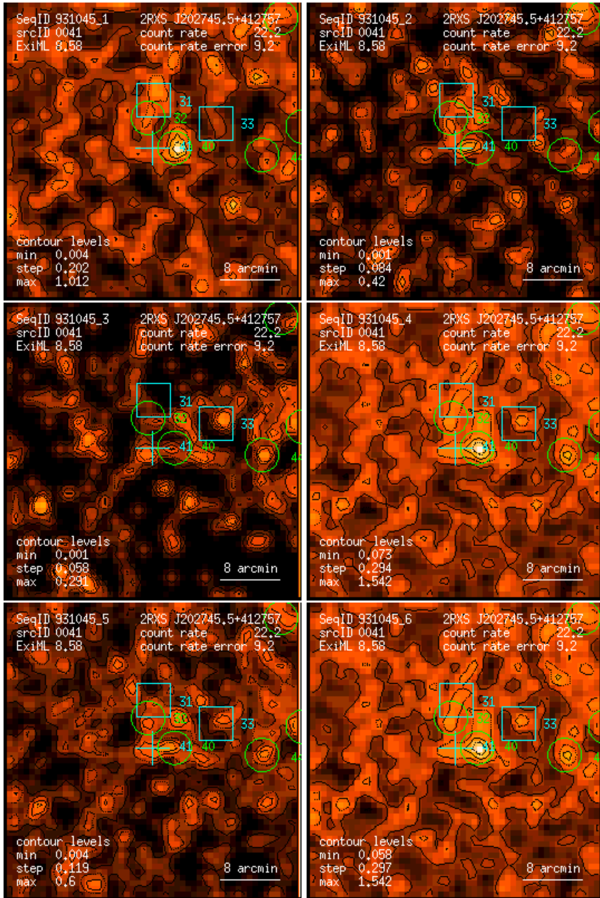
Figure 41: RASS 931045: detection 0041: band rate images, Gaussian filter: (1) PSPC channels 11 – 41, (2) 52 – 90, (3) 91 – 201, (4) 11 – 235, (5) 52 – 201, (6) 11 – 201. Broad band rates in counts/ks. Band rate contour levels in counts/ks/arcmin 2 .
