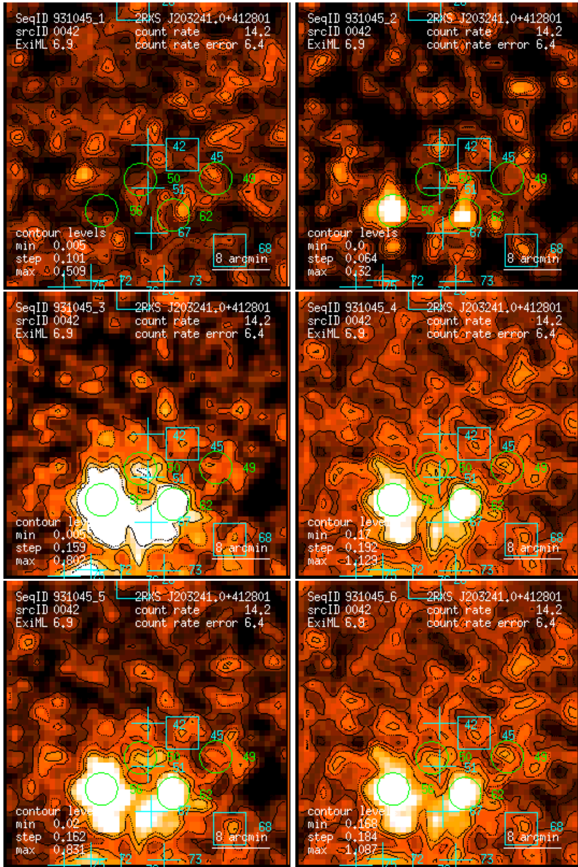
Figure 42: RASS 931045: detection 0042: band rate images, Gaussian filter: (1) PSPC channels 11 – 41, (2) 52 – 90, (3) 91 – 201, (4) 11 – 235, (5) 52 – 201, (6) 11 – 201. Broad band rates in counts/ks. Band rate contour levels in counts/ks/arcmin 2 .
