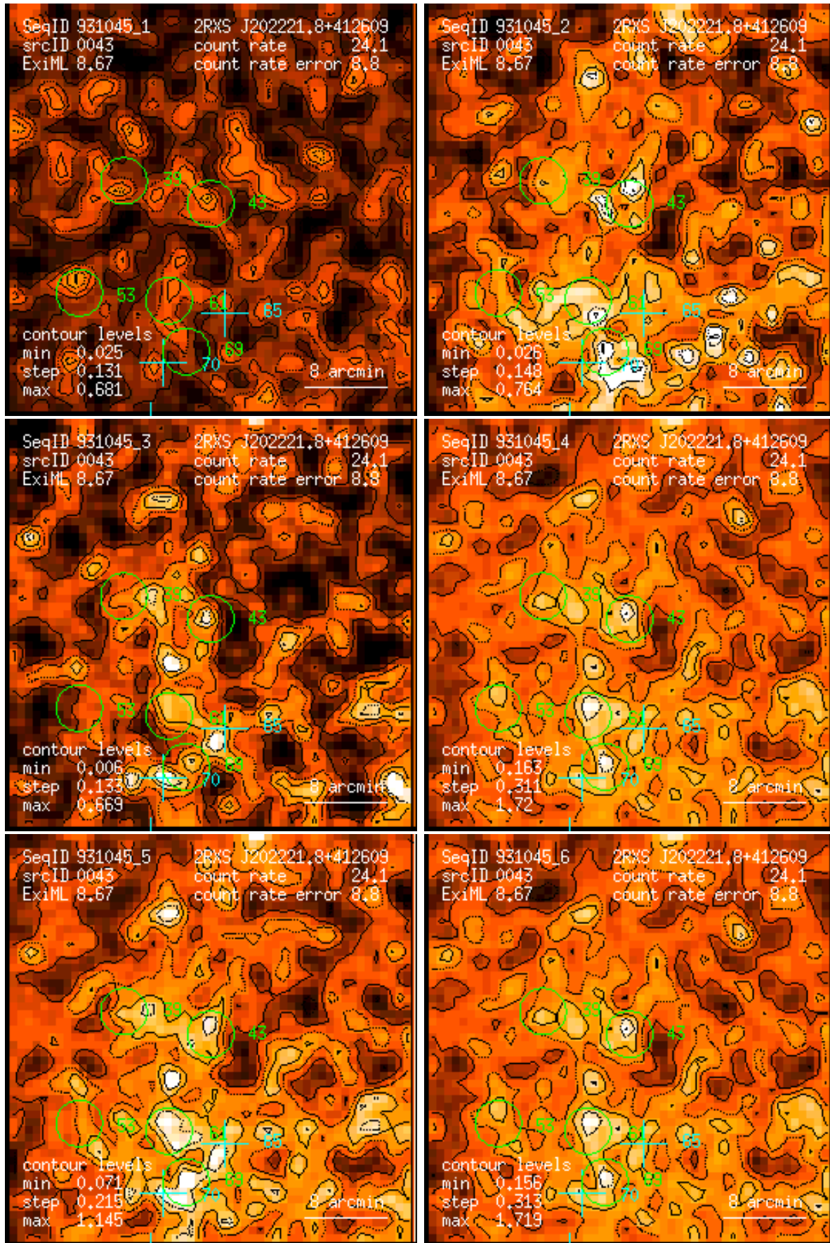
Figure 43: RASS 931045: detection 0043: band rate images, Gaussian filter: (1) PSPC channels 11 – 41, (2) 52 – 90, (3) 91 – 201, (4) 11 – 235, (5) 52 – 201, (6) 11 – 201. Broad band rates in counts/ks. Band rate contour levels in counts/ks/arcmin 2 .
