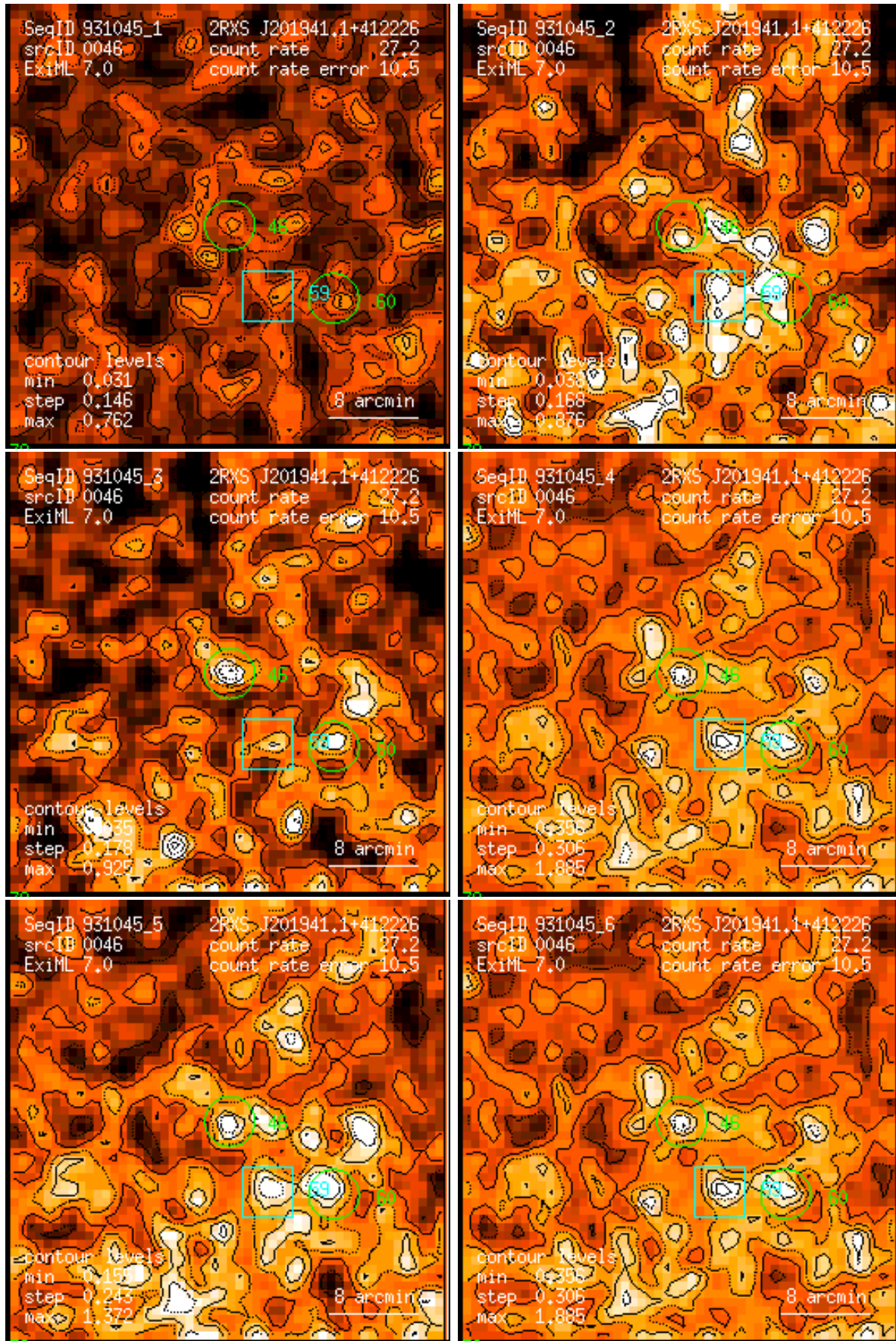
Figure 46: RASS 931045: detection 0046: band rate images, Gaussian filter: (1) PSPC channels 11 – 41, (2) 52 – 90, (3) 91 – 201, (4) 11 – 235, (5) 52 – 201, (6) 11 – 201. Broad band rates in counts/ks. Band rate contour levels in counts/ks/arcmin 2 .
