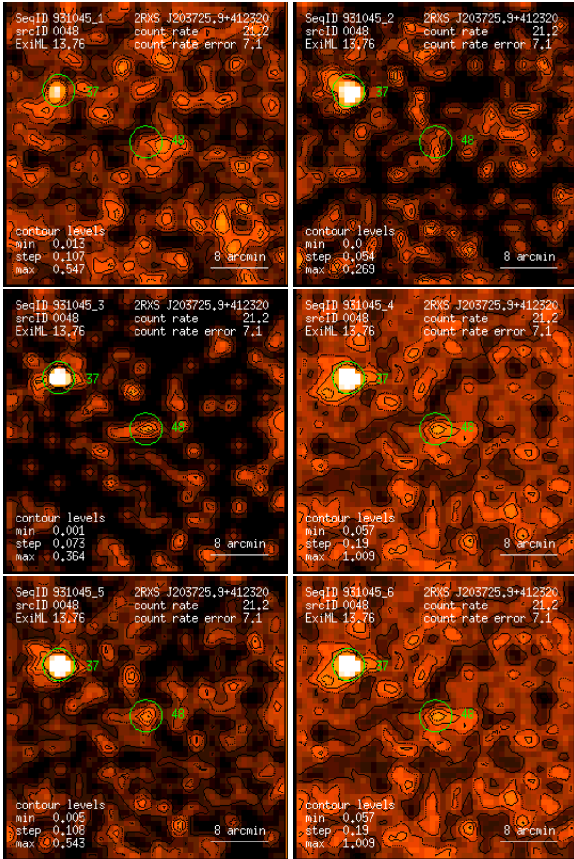
Figure 48: RASS 931045: detection 0048: band rate images, Gaussian filter: (1) PSPC channels 11 – 41, (2) 52 – 90, (3) 91 – 201, (4) 11 – 235, (5) 52 – 201, (6) 11 – 201. Broad band rates in counts/ks. Band rate contour levels in counts/ks/arcmin 2 .
