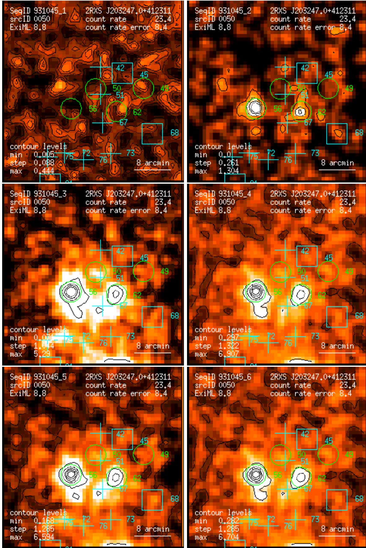
Figure 50: RASS 931045: detection 0050: band rate images, Gaussian filter: (1) PSPC channels 11 – 41, (2) 52 – 90, (3) 91 – 201, (4) 11 – 235, (5) 52 – 201, (6) 11 – 201. Broad band rates in counts/ks. Band rate contour levels in counts/ks/arcmin 2 .
