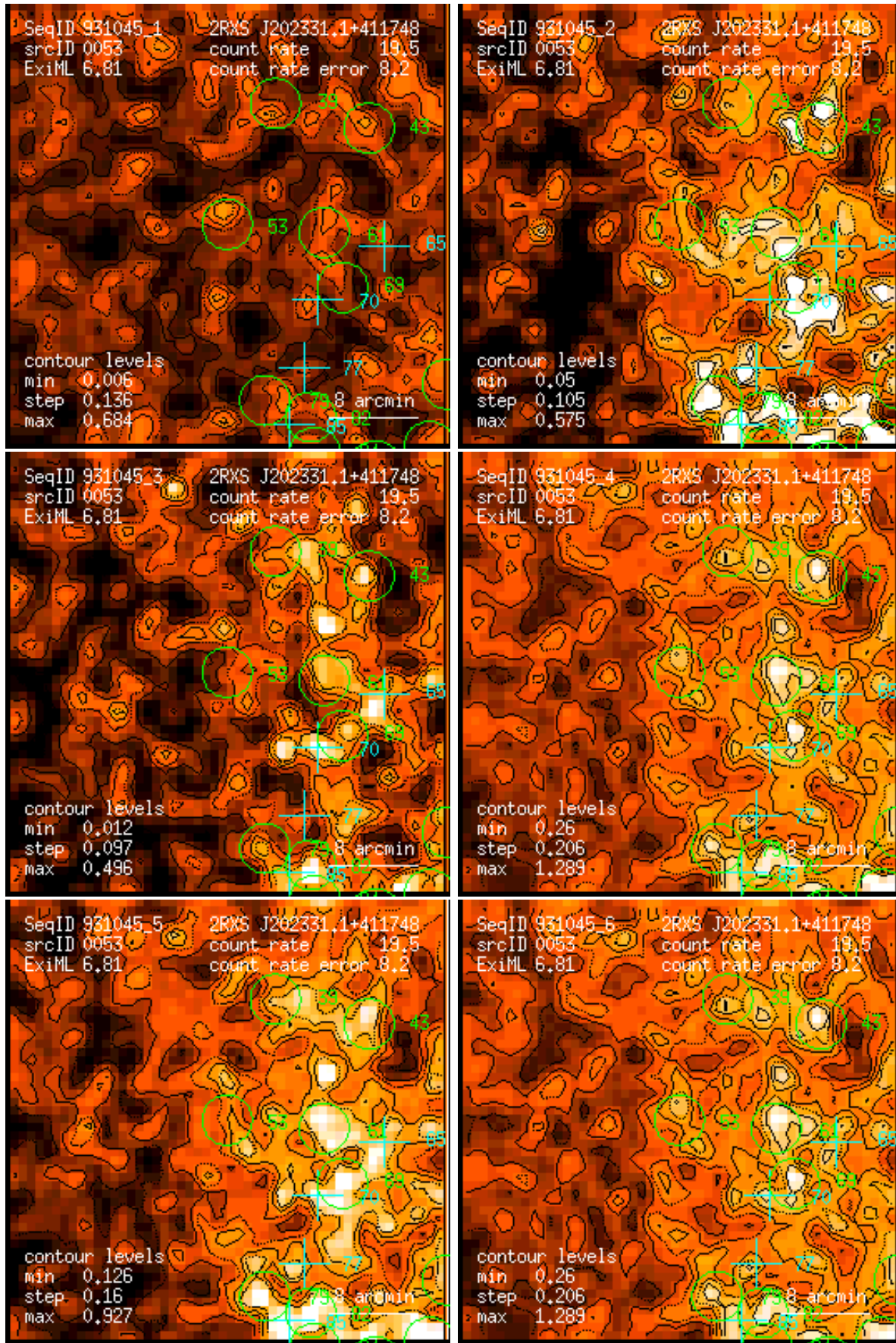
Figure 53: RASS 931045: detection 0053: band rate images, Gaussian filter: (1) PSPC channels 11 – 41, (2) 52 – 90, (3) 91 – 201, (4) 11 – 235, (5) 52 – 201, (6) 11 – 201. Broad band rates in counts/ks. Band rate contour levels in counts/ks/arcmin 2 .
