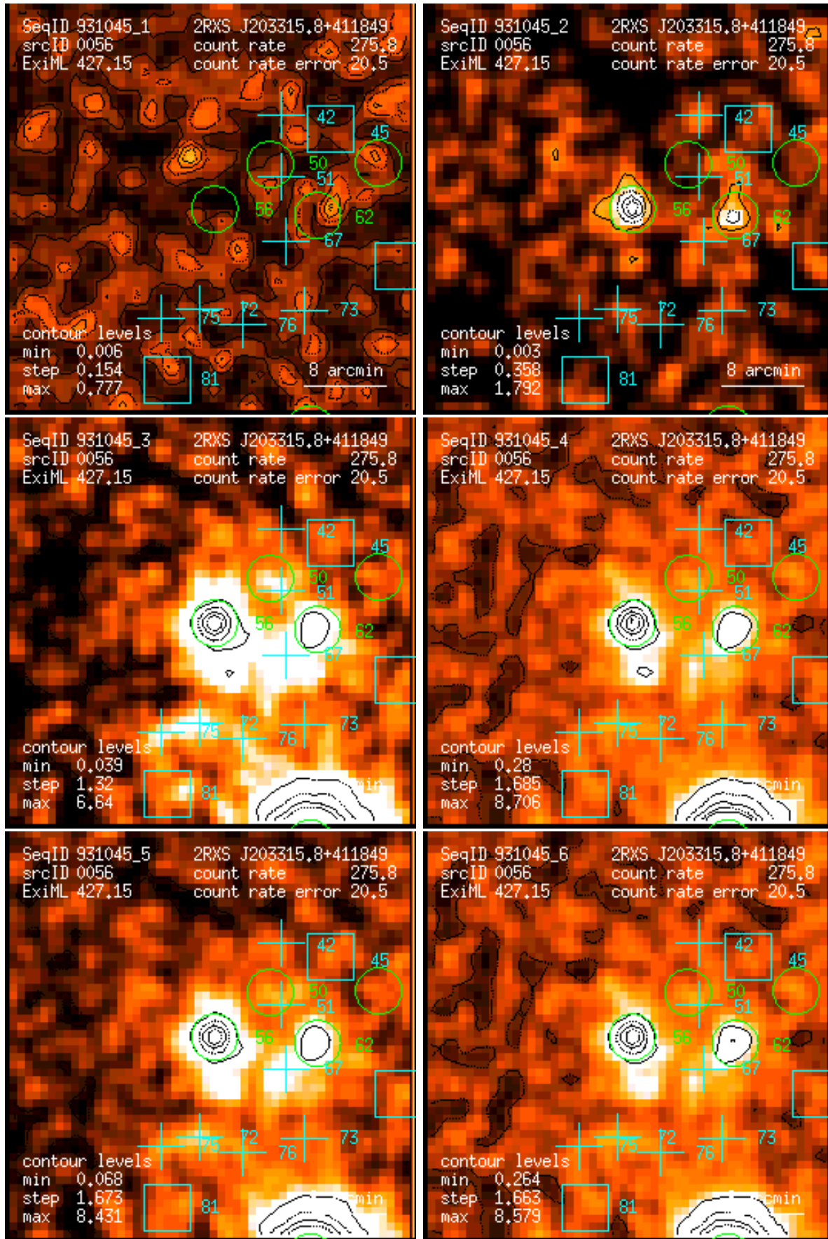
Figure 56: RASS 931045: detection 0056: band rate images, Gaussian filter: (1) PSPC channels 11 – 41, (2) 52 – 90, (3) 91 – 201, (4) 11 – 235, (5) 52 – 201, (6) 11 – 201. Broad band rates in counts/ks. Band rate contour levels in counts/ks/arcmin 2 .
