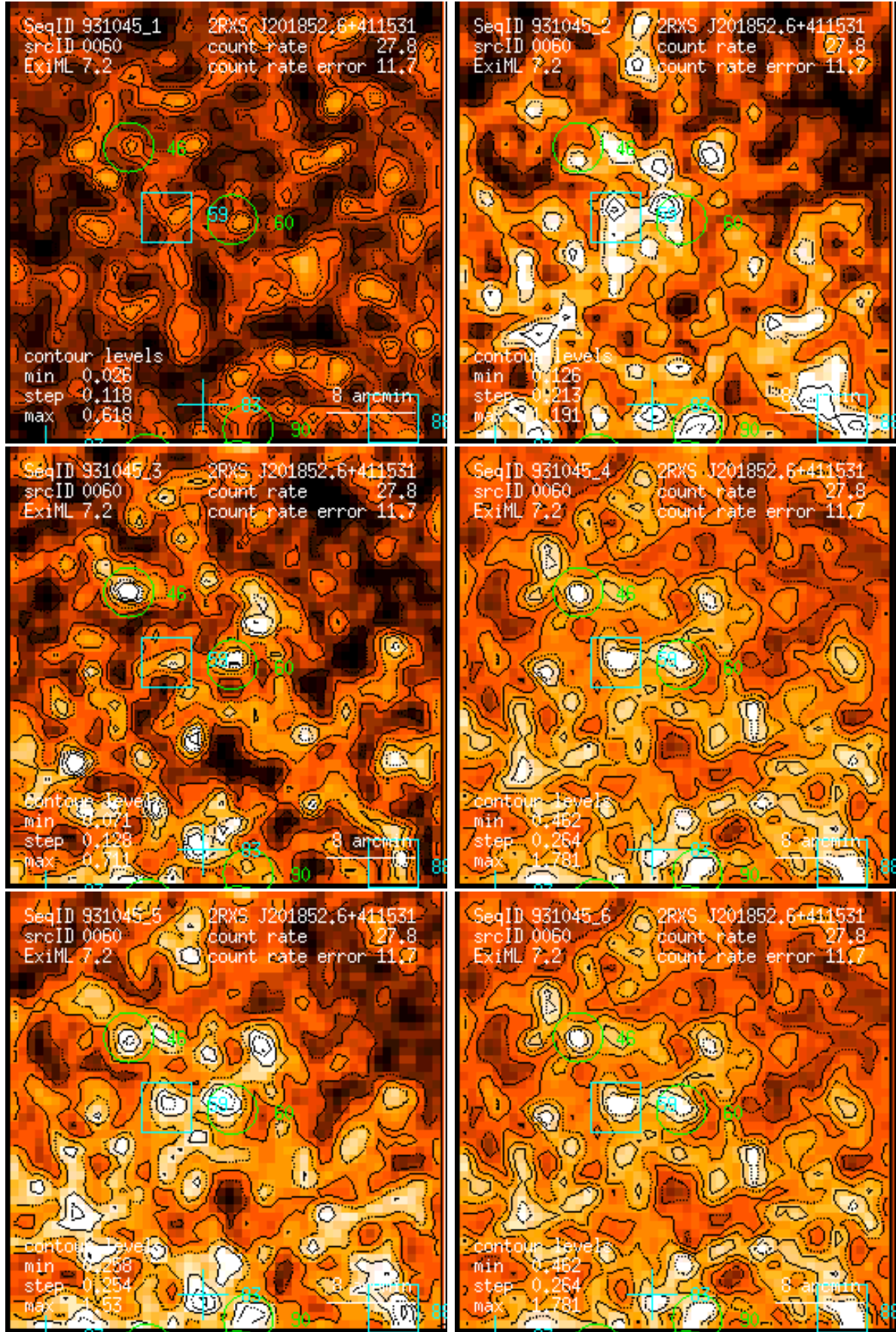
Figure 60: RASS 931045: detection 0060: band rate images, Gaussian filter: (1) PSPC channels 11 – 41, (2) 52 – 90, (3) 91 – 201, (4) 11 – 235, (5) 52 – 201, (6) 11 – 201. Broad band rates in counts/ks. Band rate contour levels in counts/ks/arcmin 2 .
