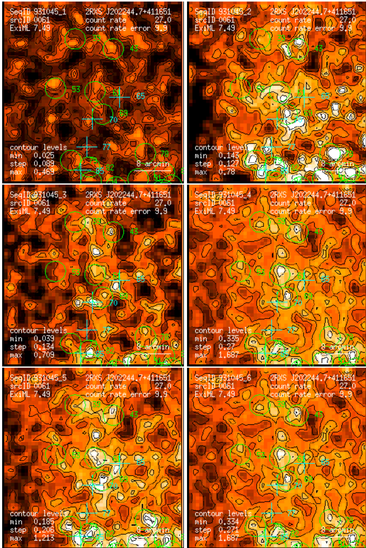
Figure 61: RASS 931045: detection 0061: band rate images, Gaussian filter: (1) PSPC channels 11 – 41, (2) 52 – 90, (3) 91 – 201, (4) 11 – 235, (5) 52 – 201, (6) 11 – 201. Broad band rates in counts/ks. Band rate contour levels in counts/ks/arcmin 2 .
