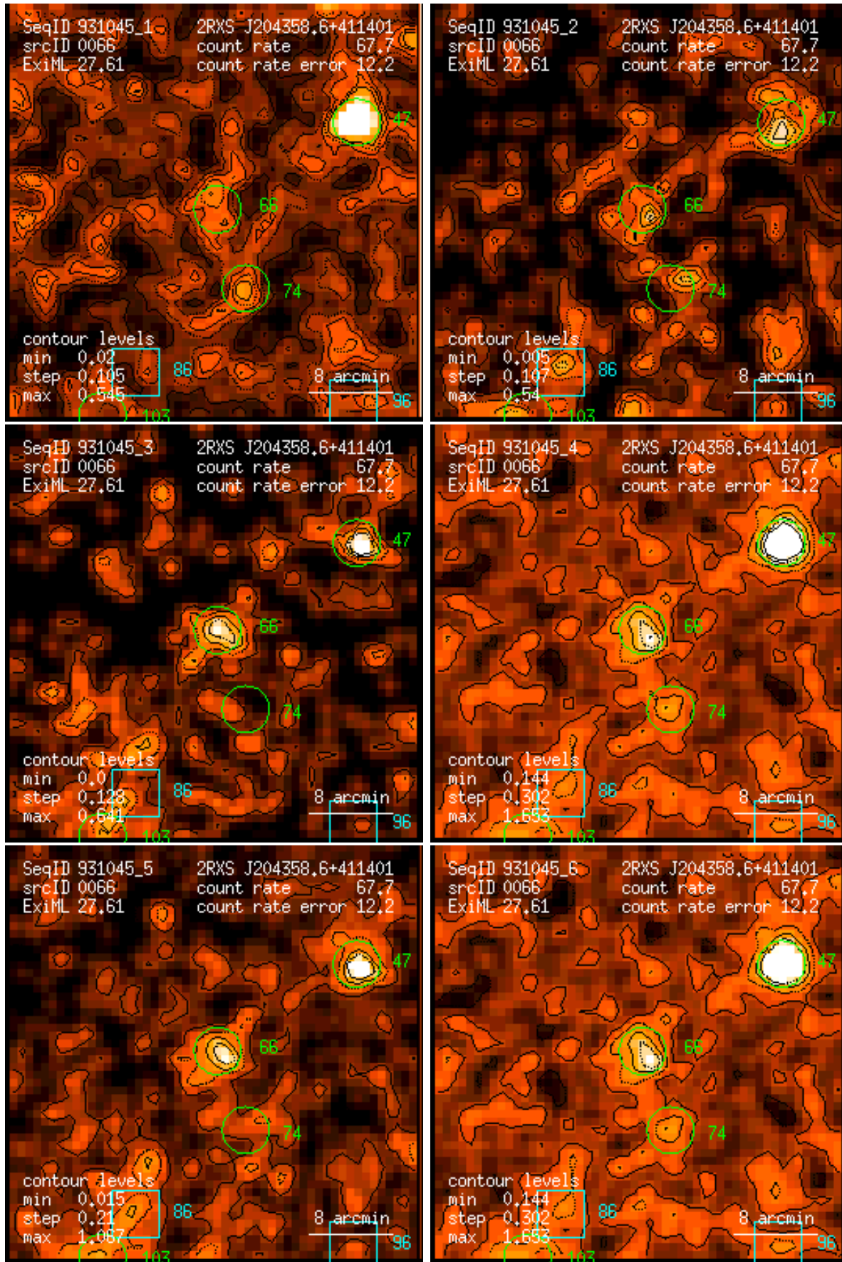
Figure 66: RASS 931045: detection 0066: band rate images, Gaussian filter: (1) PSPC channels 11 – 41, (2) 52 – 90, (3) 91 – 201, (4) 11 – 235, (5) 52 – 201, (6) 11 – 201. Broad band rates in counts/ks. Band rate contour levels in counts/ks/arcmin 2 .
