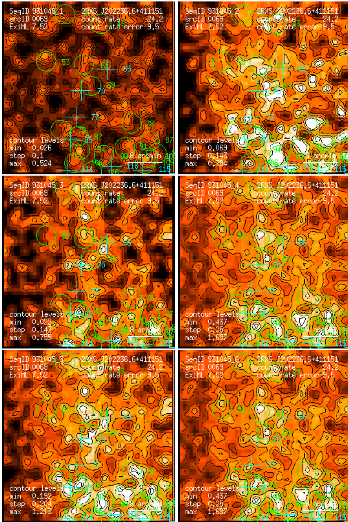
Figure 69: RASS 931045: detection 0069: band rate images, Gaussian filter: (1) PSPC channels 11 – 41, (2) 52 – 90, (3) 91 – 201, (4) 11 – 235, (5) 52 – 201, (6) 11 – 201. Broad band rates in counts/ks. Band rate contour levels in counts/ks/arcmin 2 .
