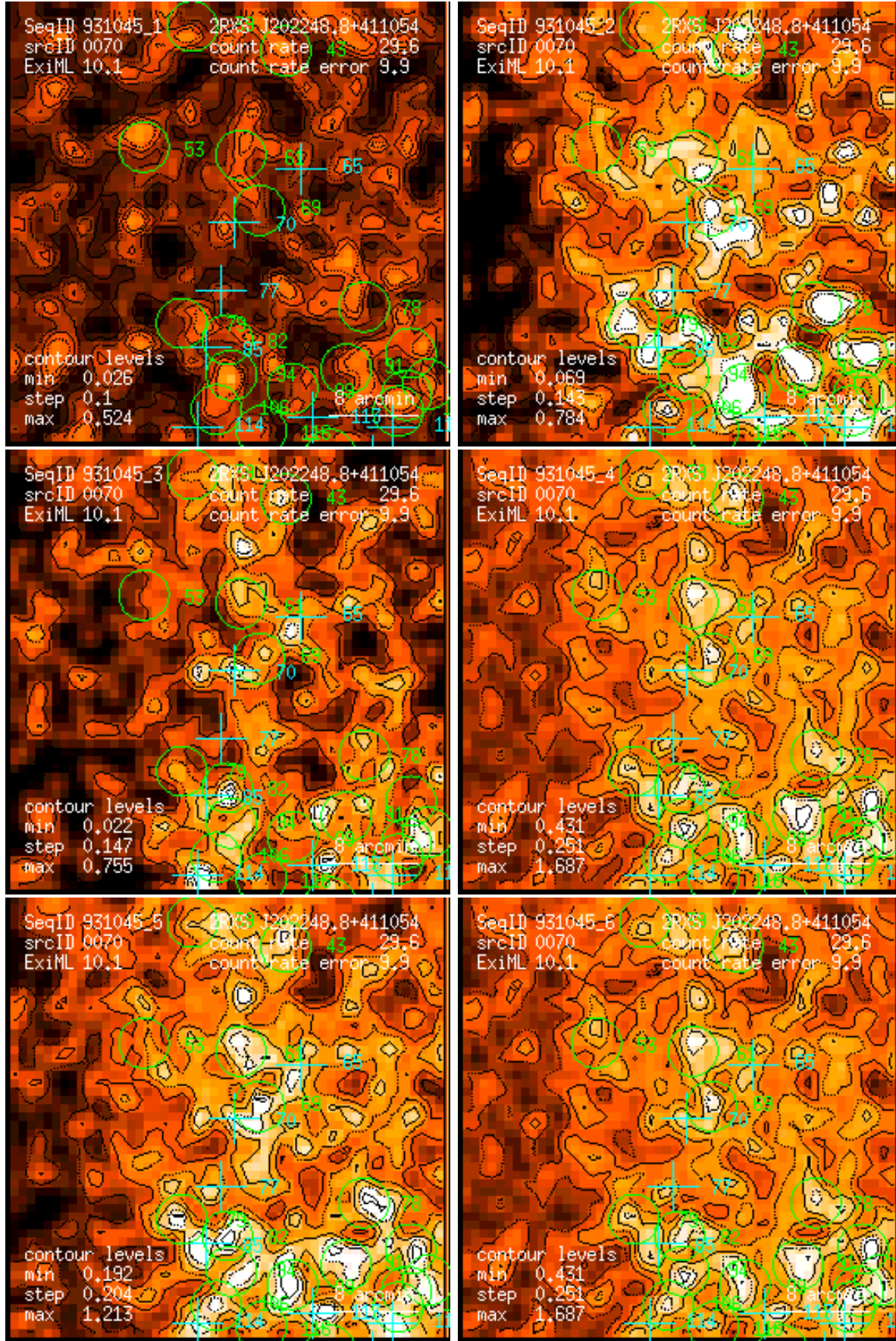
Figure 70: RASS 931045: detection 0070: band rate images, Gaussian filter: (1) PSPC channels 11 – 41, (2) 52 – 90, (3) 91 – 201, (4) 11 – 235, (5) 52 – 201, (6) 11 – 201. Broad band rates in counts/ks. Band rate contour levels in counts/ks/arcmin 2 .
